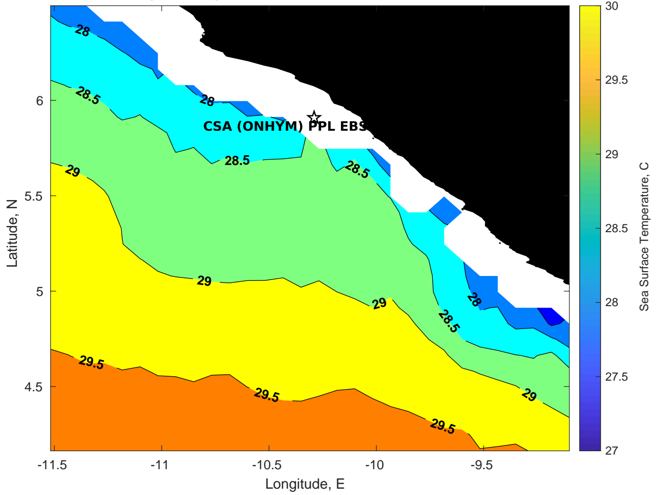
SST for CSA (ONHYM) PPL EBS - Liberia at 18-Feb-2025 00:00:00
