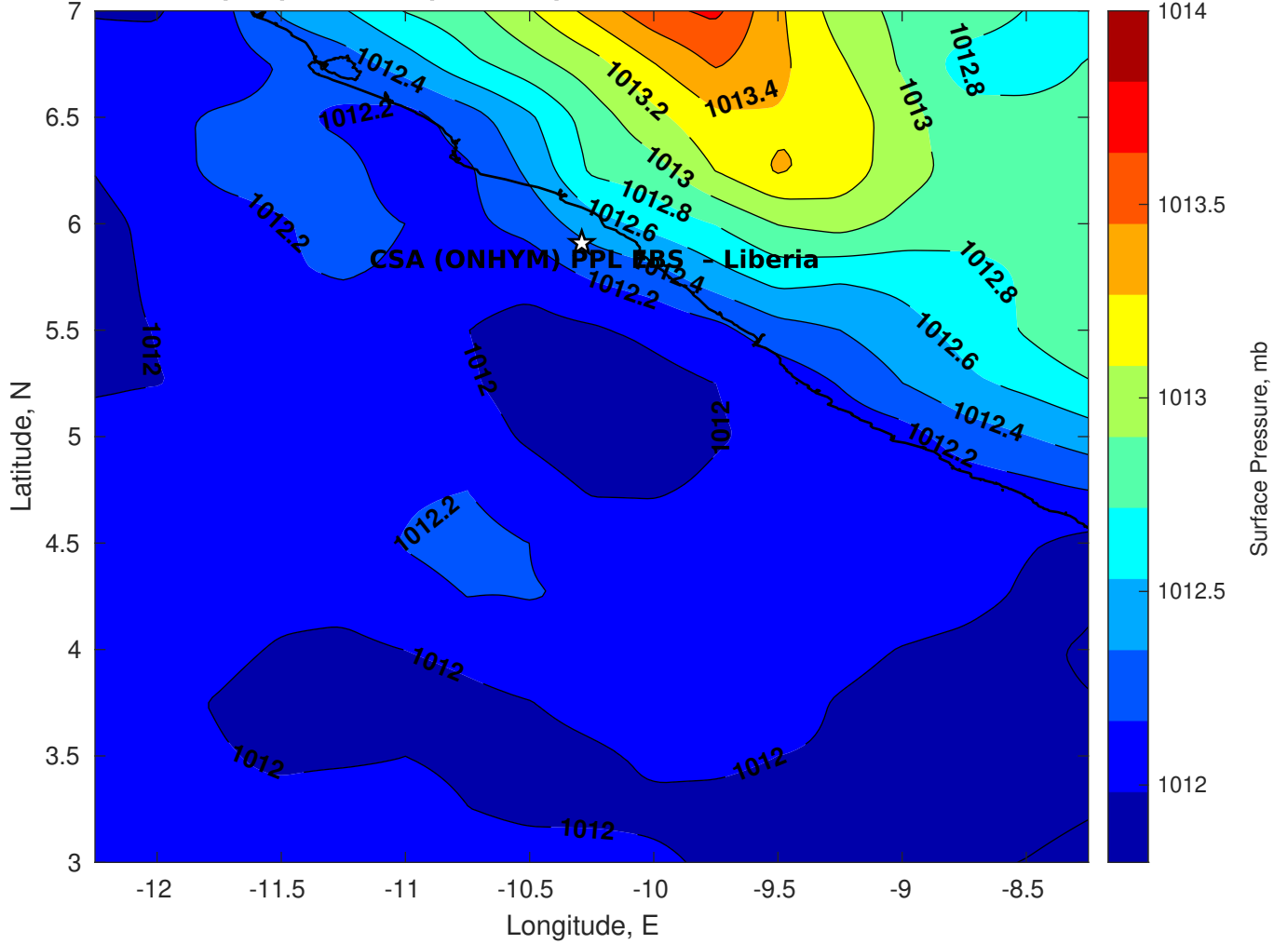
Surface Pressure (mb) for CSA (ONHYM) PPL EBS - Liberia at 21-Feb-2025 00:00:00
