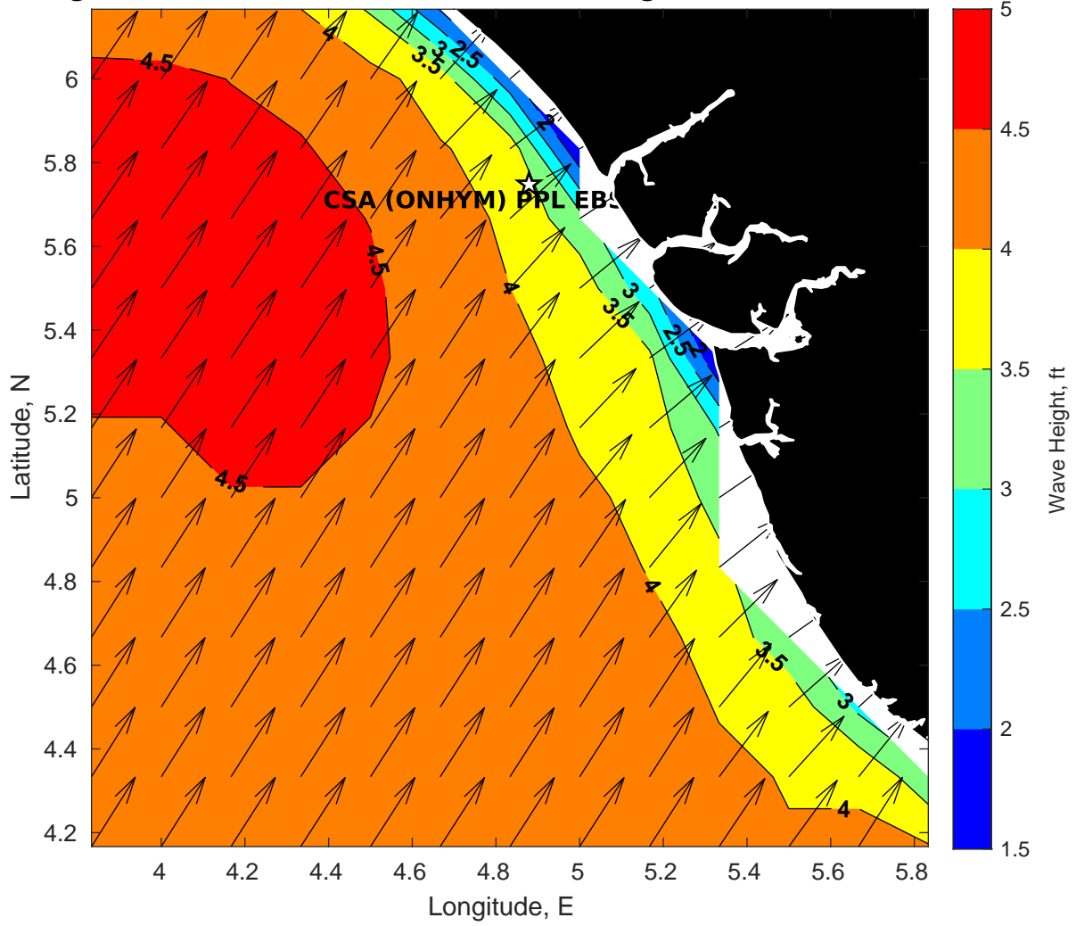
Wave Height (ft) for CSA (ONHYM) PPL EBS - Nigeria at 19-Feb-2025 09:00:00
