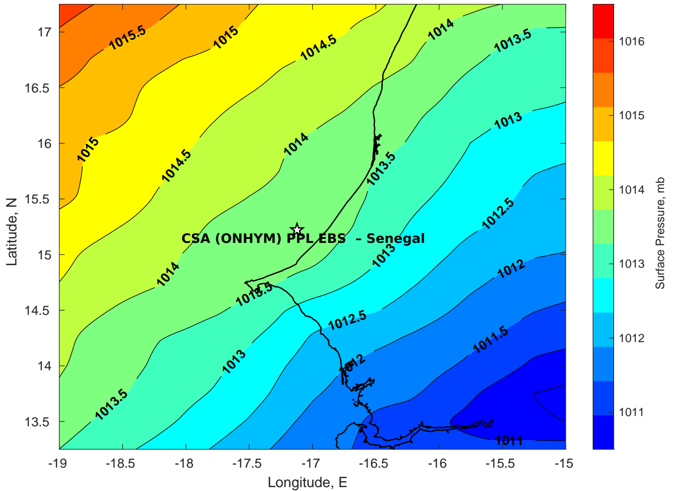
Surface Pressure (mb) for CSA (ONHYM) PPL EBS - Senegal at 20-Feb-2025 00:00:00
