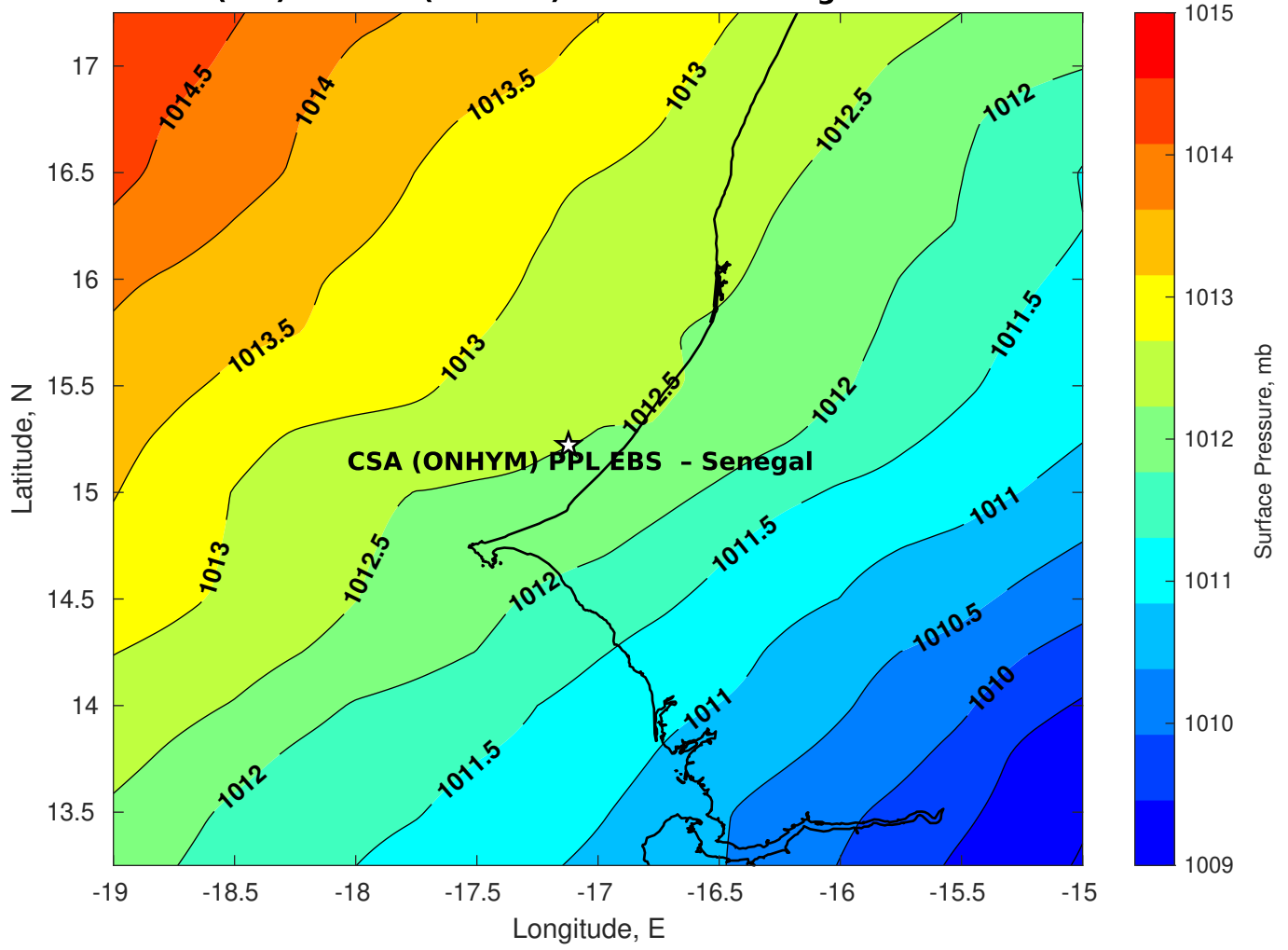
Surface Pressure (mb) for CSA (ONHYM) PPL EBS - Senegal at 19-Feb-2025 00:00:00
