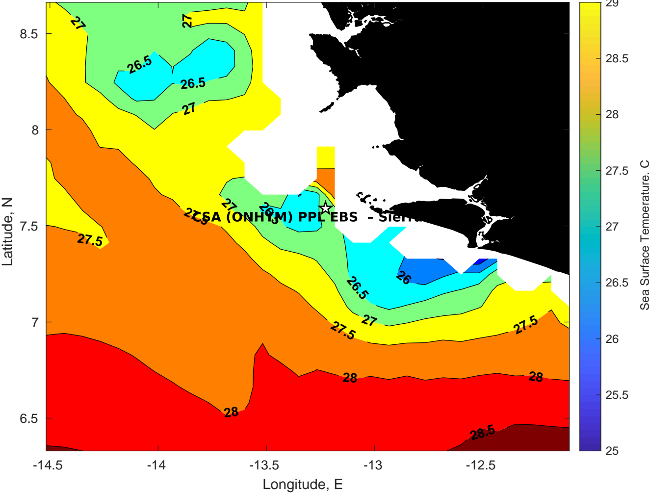
SST for CSA (ONHYM) PPL EBS - Sierra Leone at 18-Feb-2025 00:00:00
