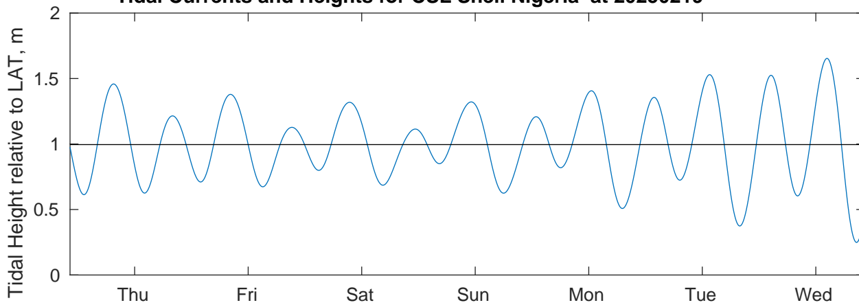
Tidal Currents and Heights for CSL Shell Nigeria at 20250219
