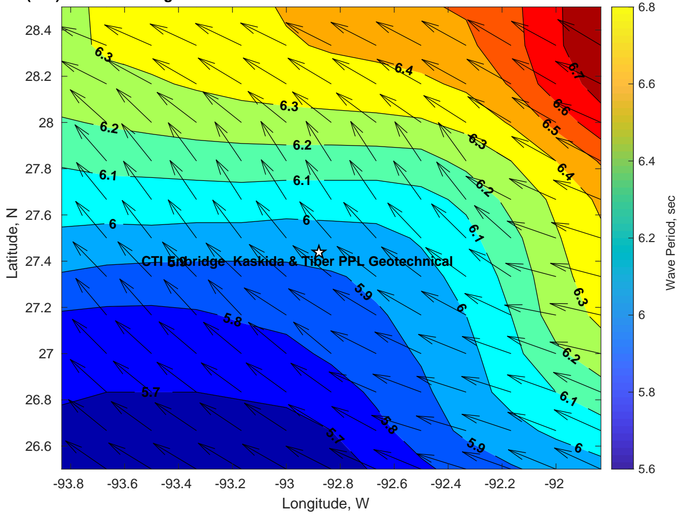
Wave Period (sec) for CTI Enbridge Kaskida & Tiber PPL Geotechnical at 19-Feb-2025 09:00:00
