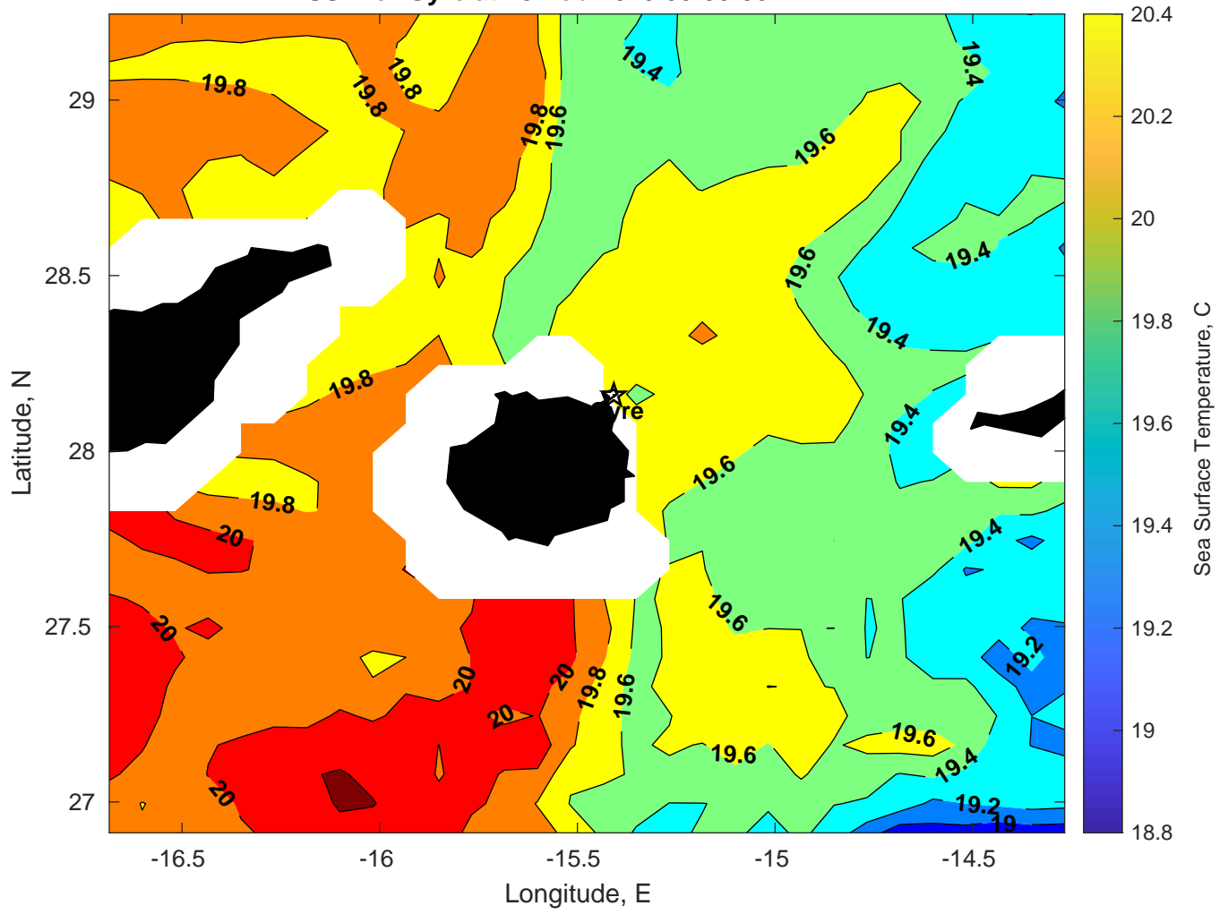
SST for Gyre at 18-Feb-2025 00:00:00
