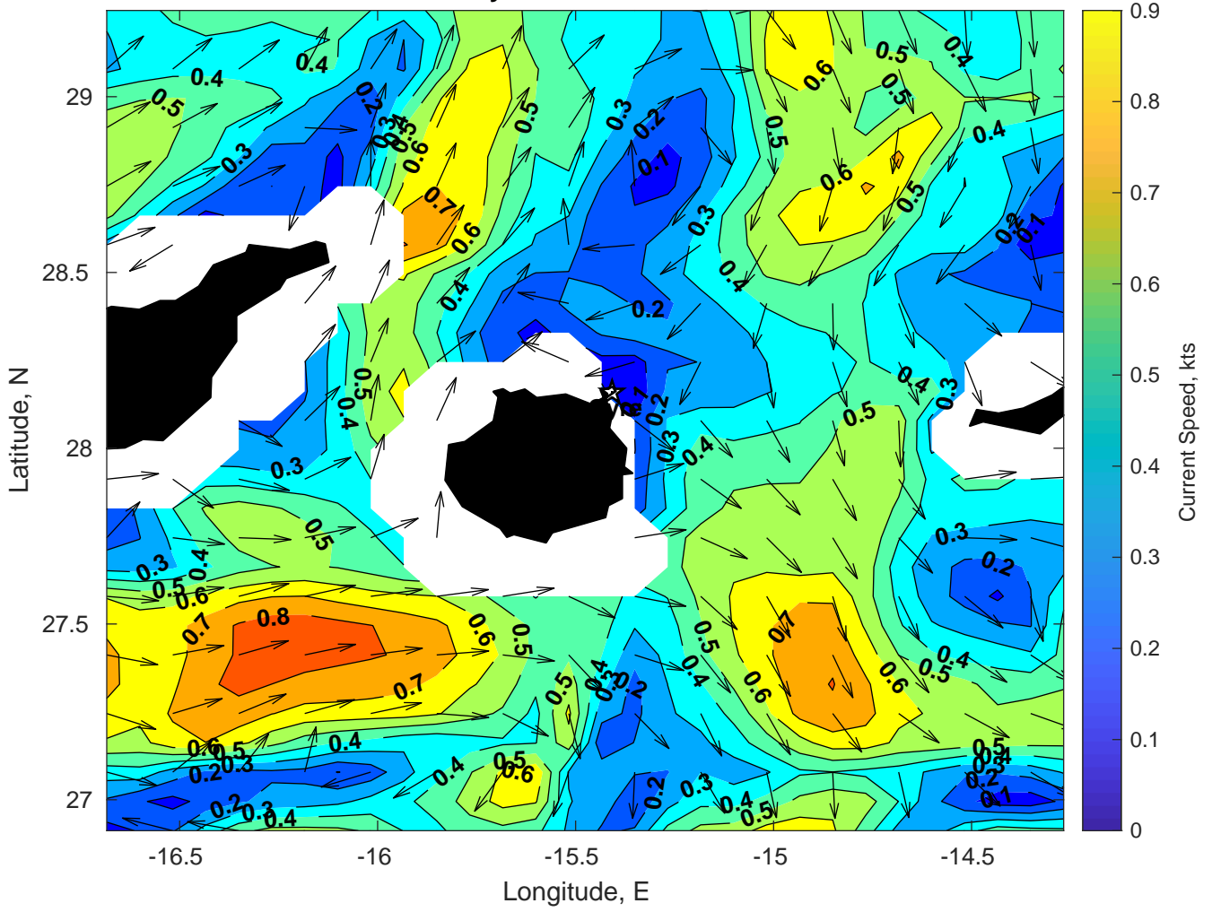
Surface Currents for Gyre at 18-Feb-2025 00:00:00
