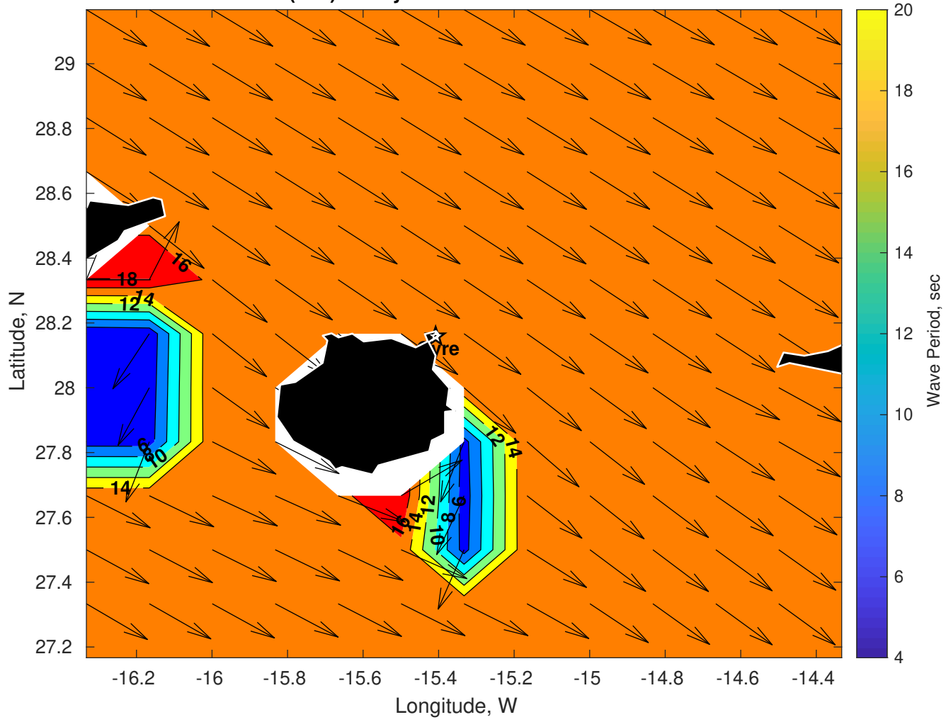
Wave Period (sec) for Gyre at 19-Feb-2025 09:00:00
