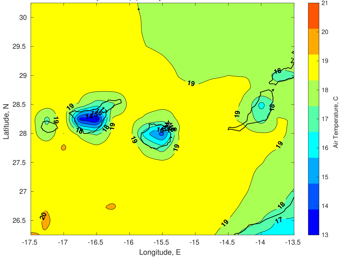
Air Temperature (C) for Gyre at 19-Feb-2025
