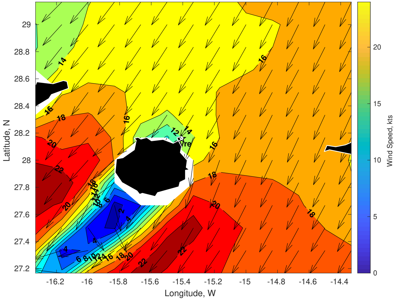
Winds (kts) for Gyre at 19-Feb-2025 09:00:00
