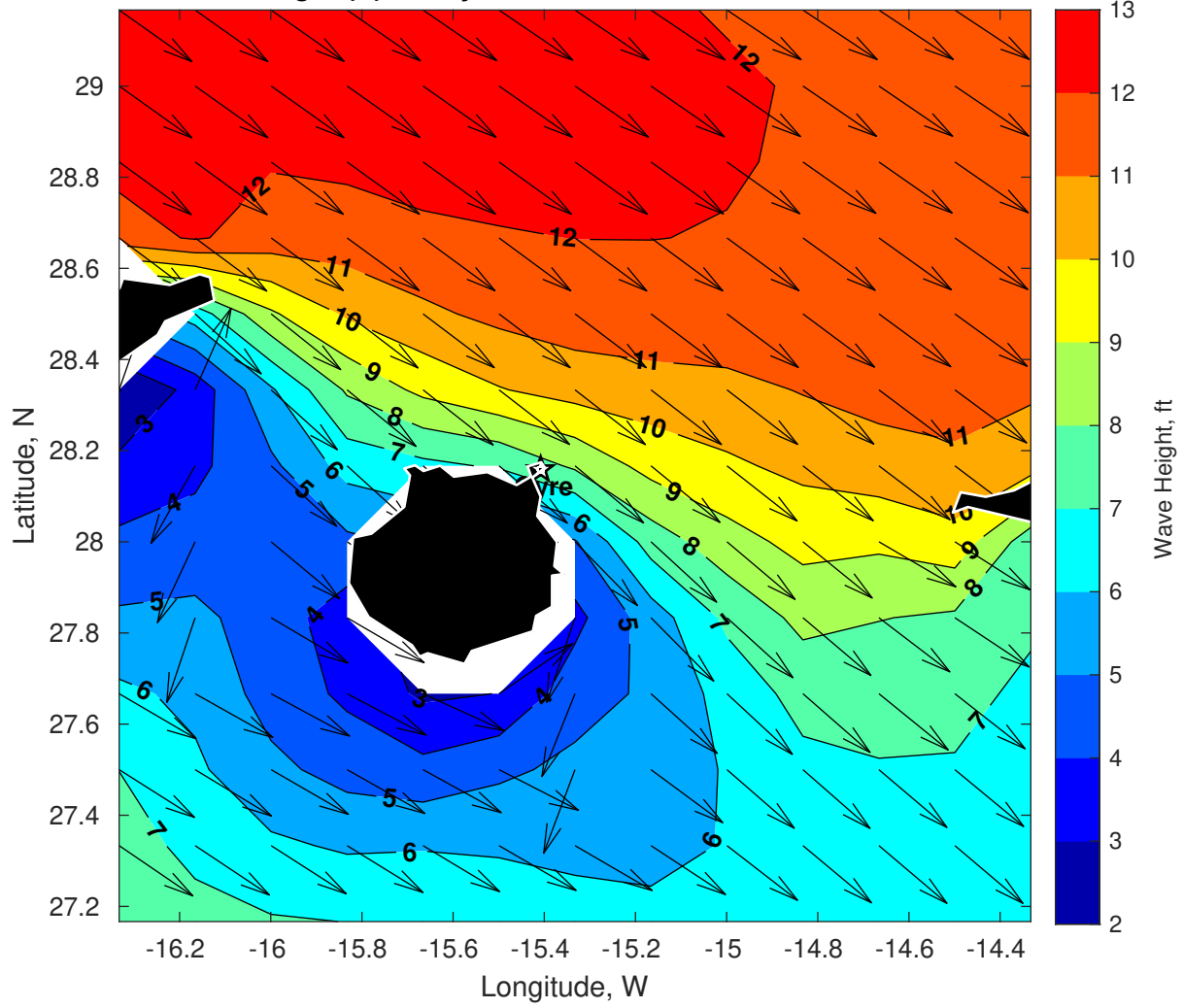
Wave Height (ft) for Gyre at 19-Feb-2025 09:00:00
