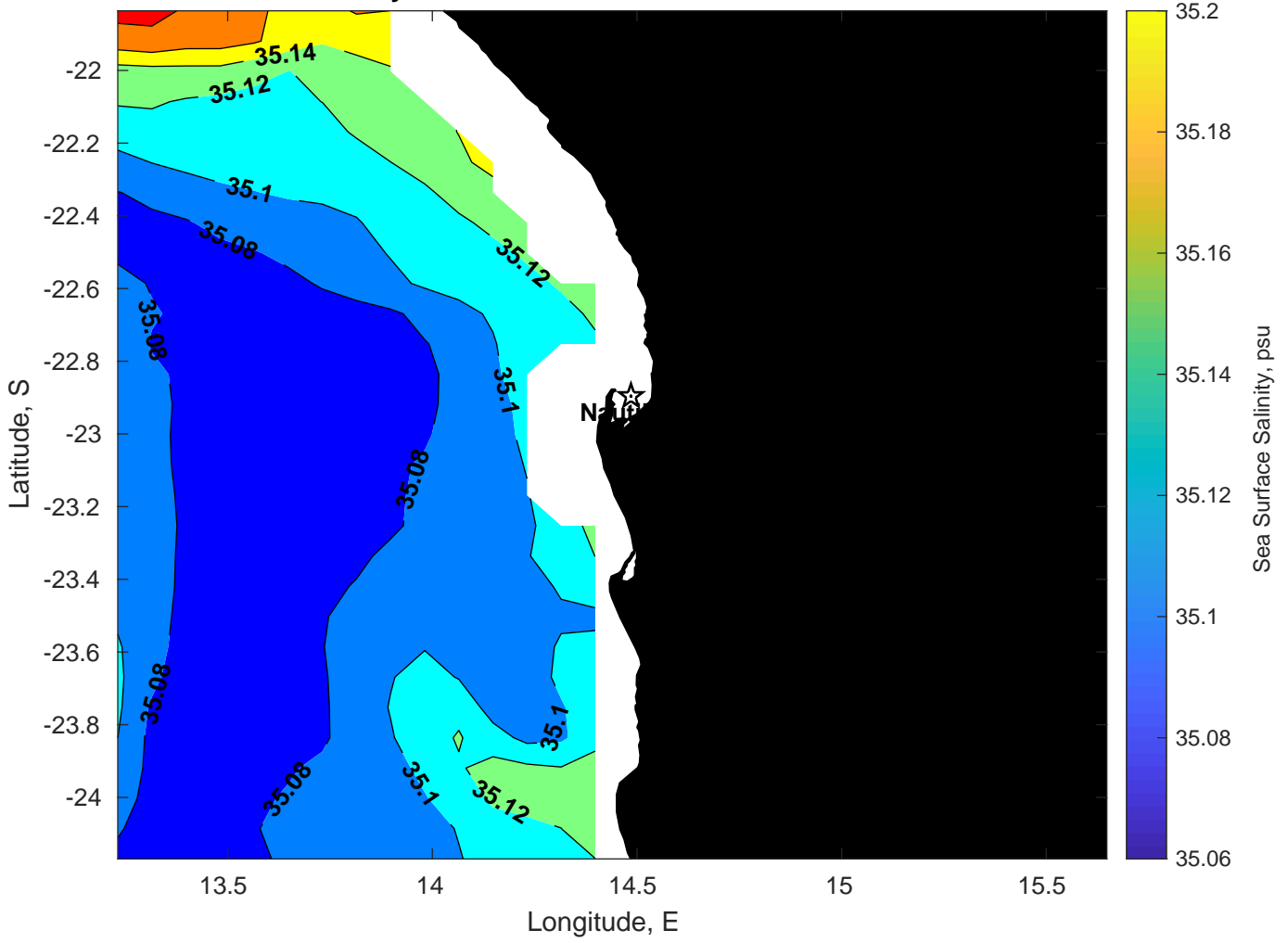
Surface Salinity for Nautilus at 18-Feb-2025 00:00:00
