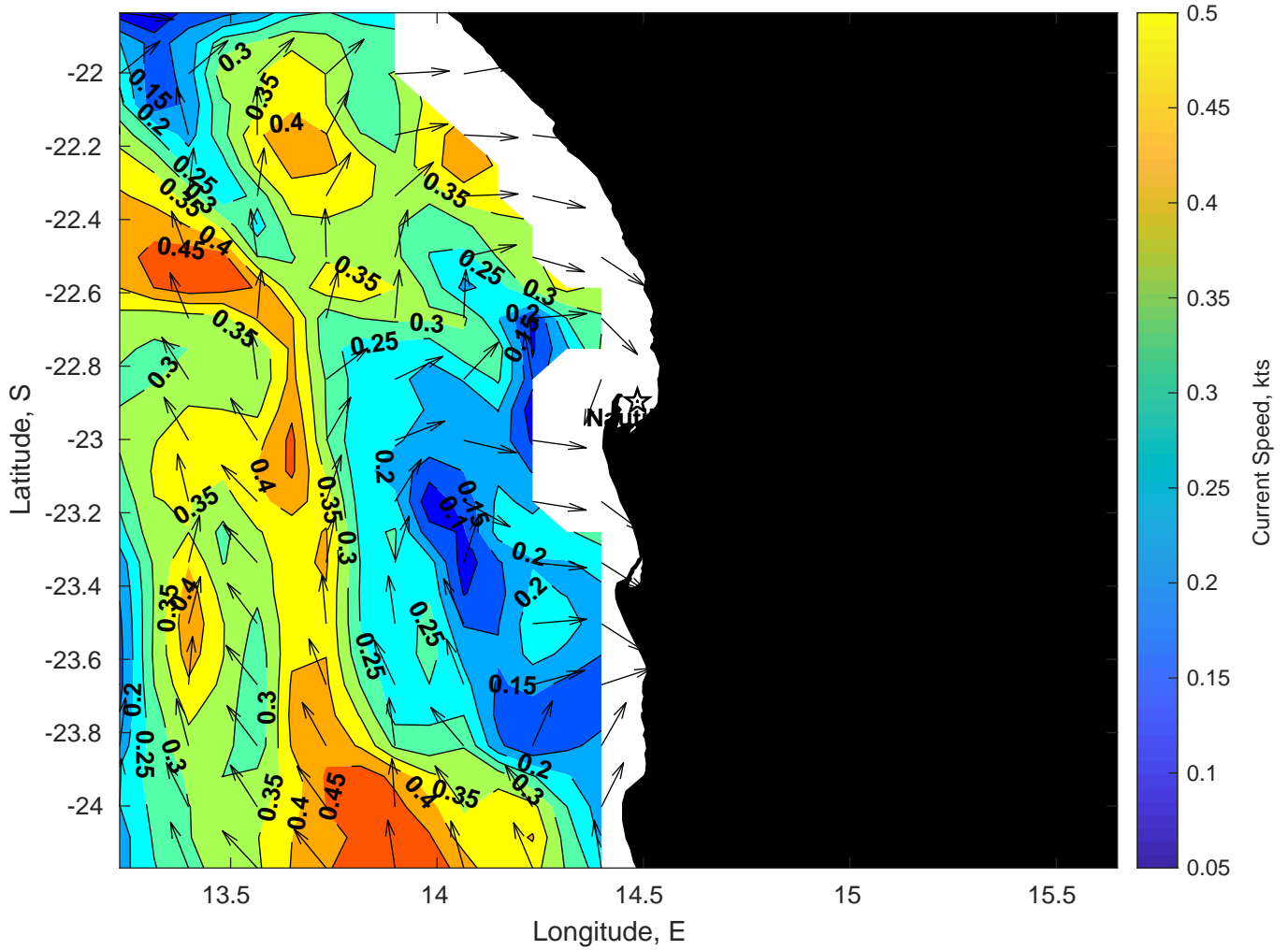
Surface Currents for Nautilus at 18-Feb-2025 00:00:00
