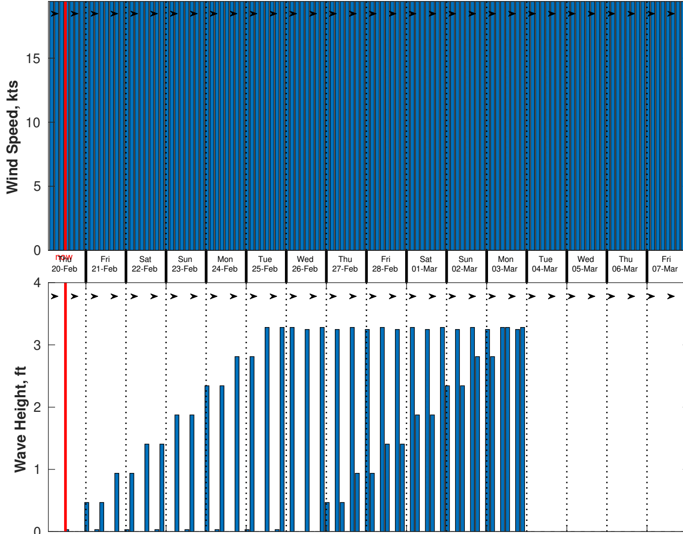
Wind & Wave Forecast for Nautilus from 19-Feb-2025 02:00:00 to 07-Mar-2025 02:00:00
