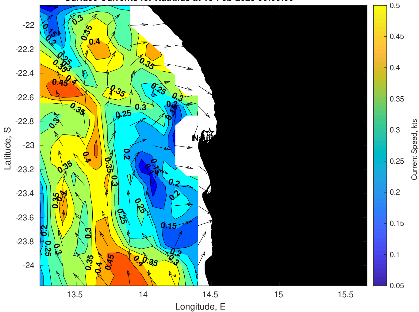
Surface Currents for Nautilus at 18-Feb-2025 00:00:00
