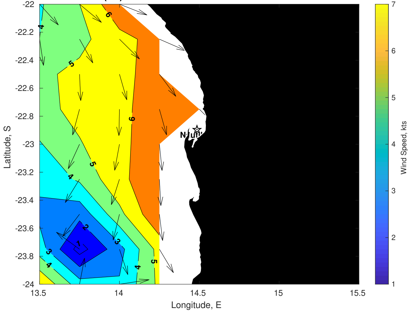
Winds (kts) for Nautilus at 19-Feb-2025 09:00:00
