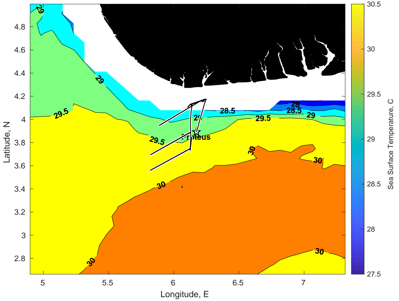
SST for Proteus at 18-Feb-2025 00:00:00
