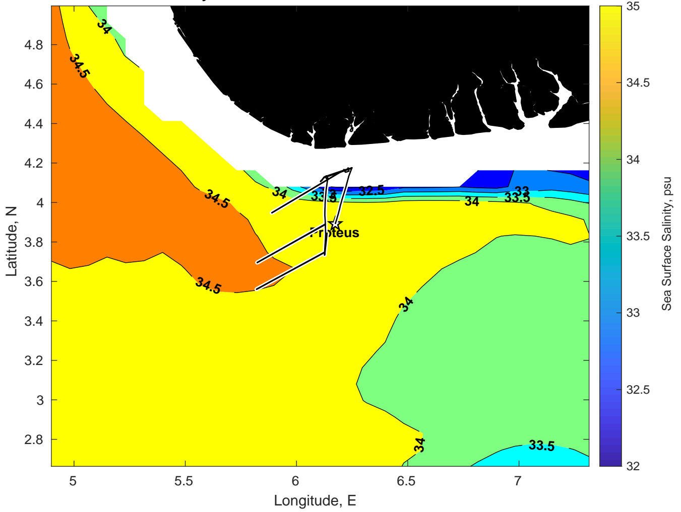
Surface Salinity for Proteus at 18-Feb-2025 00:00:00
