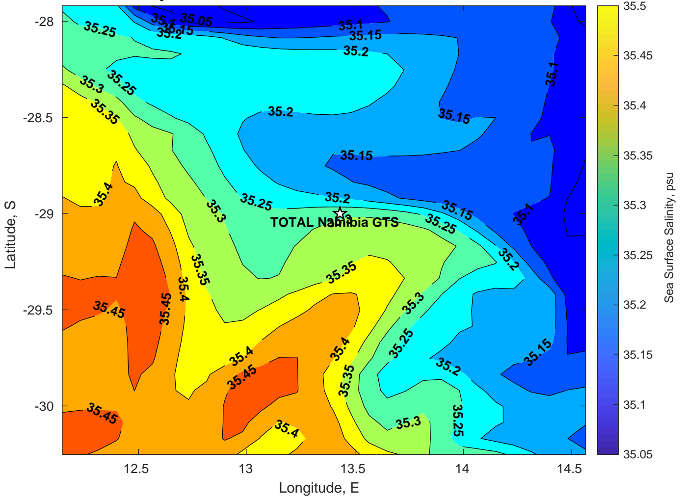
Surface Salinity for TOTAL Namibia GTS at 18-Feb-2025 00:00:00
