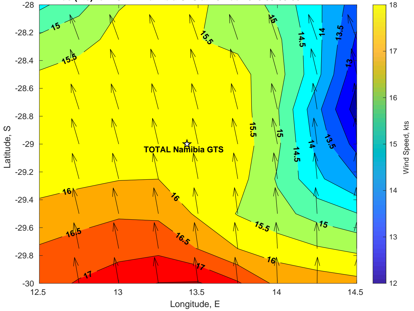
Winds (kts) for TOTAL Namibia GTS at 19-Feb-2025 09:00:00
