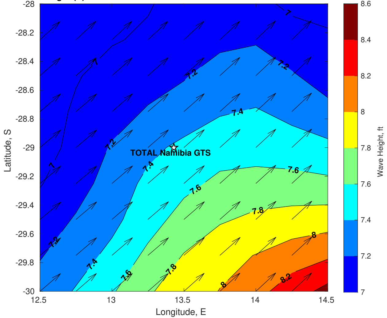
Wave Height (ft) for TOTAL Namibia GTS at 19-Feb-2025 09:00:00
