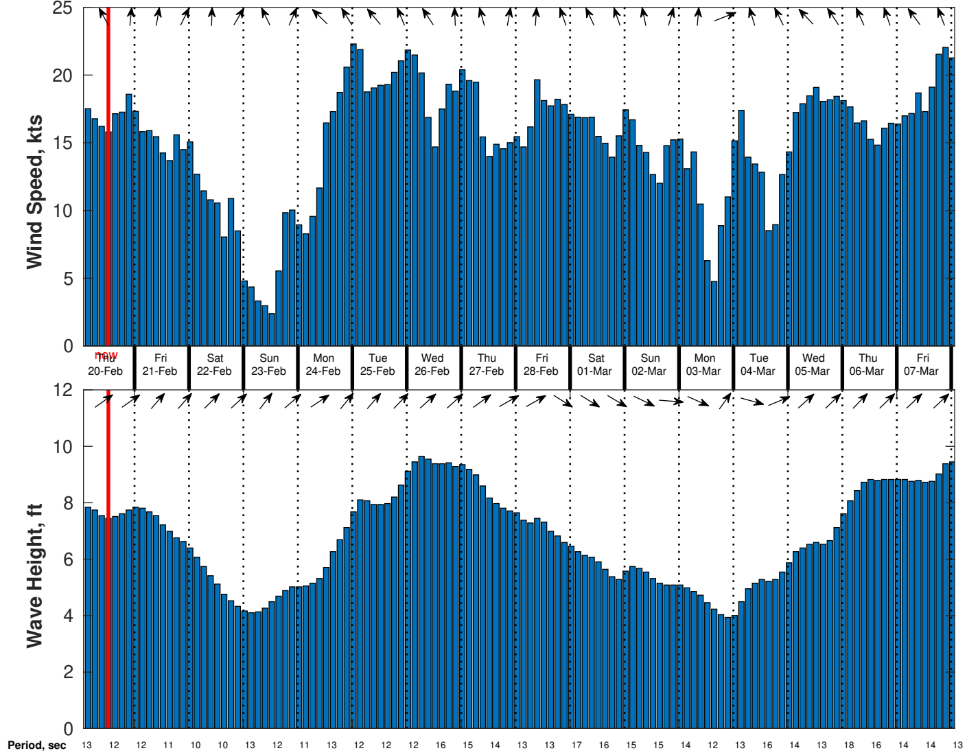
Wind & Wave Forecast for TOTAL Namibia GTS from 19-Feb-2025 02:00:00 to 07-Mar-2025 02:00:00
