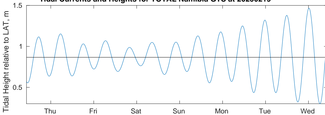
Tidal Currents and Heights for TOTAL Namibia GTS at 20250219
