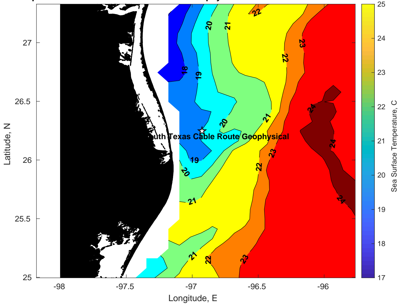
SST for Tampnet P2378 South Texas Cable Route Geophysical at 18-Feb-2025 00:00:00
