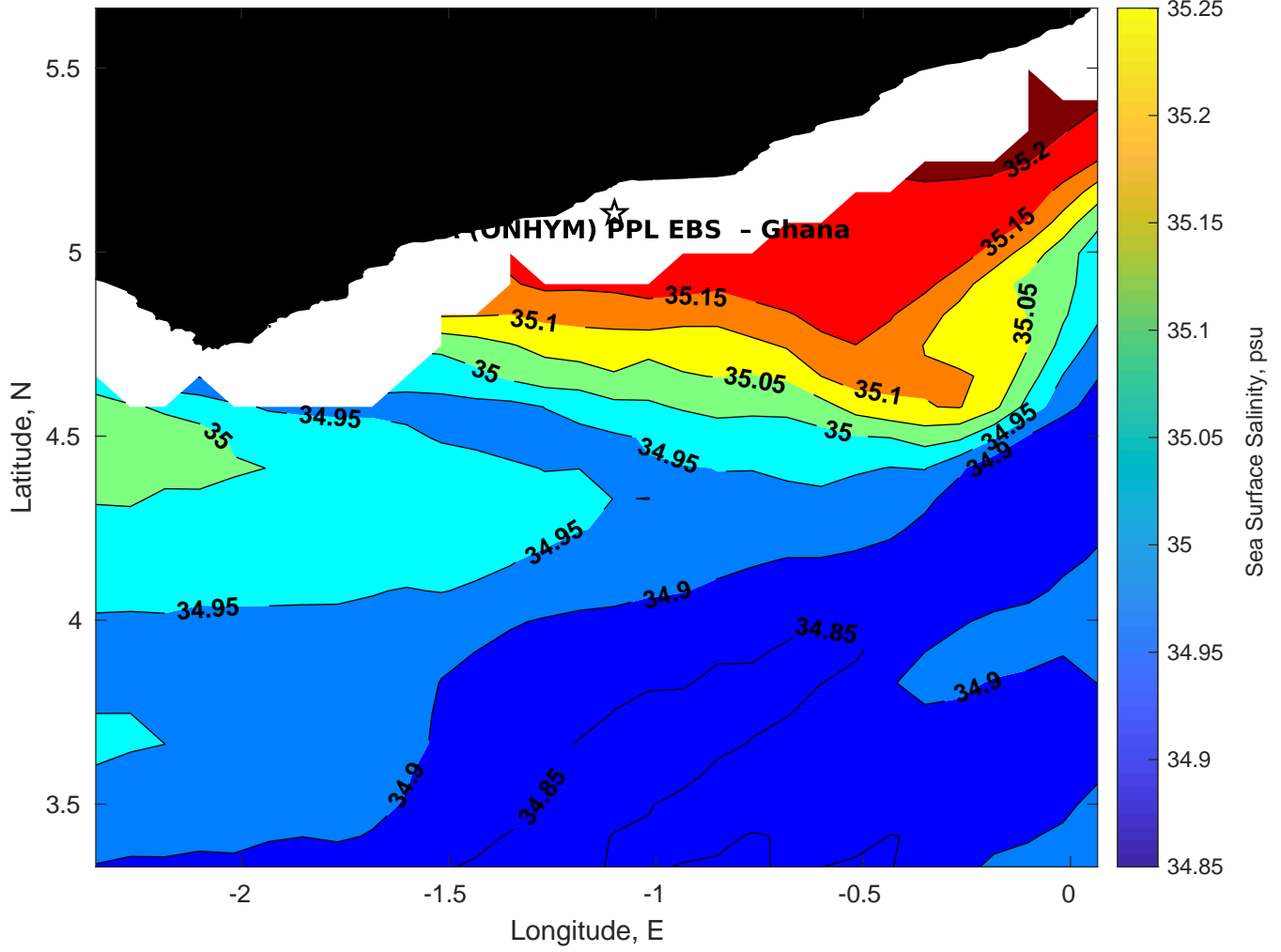
Surface Salinity for CSA (ONHYM) PPL EBS - Ghana at 19-Feb-2025 00:00:00
