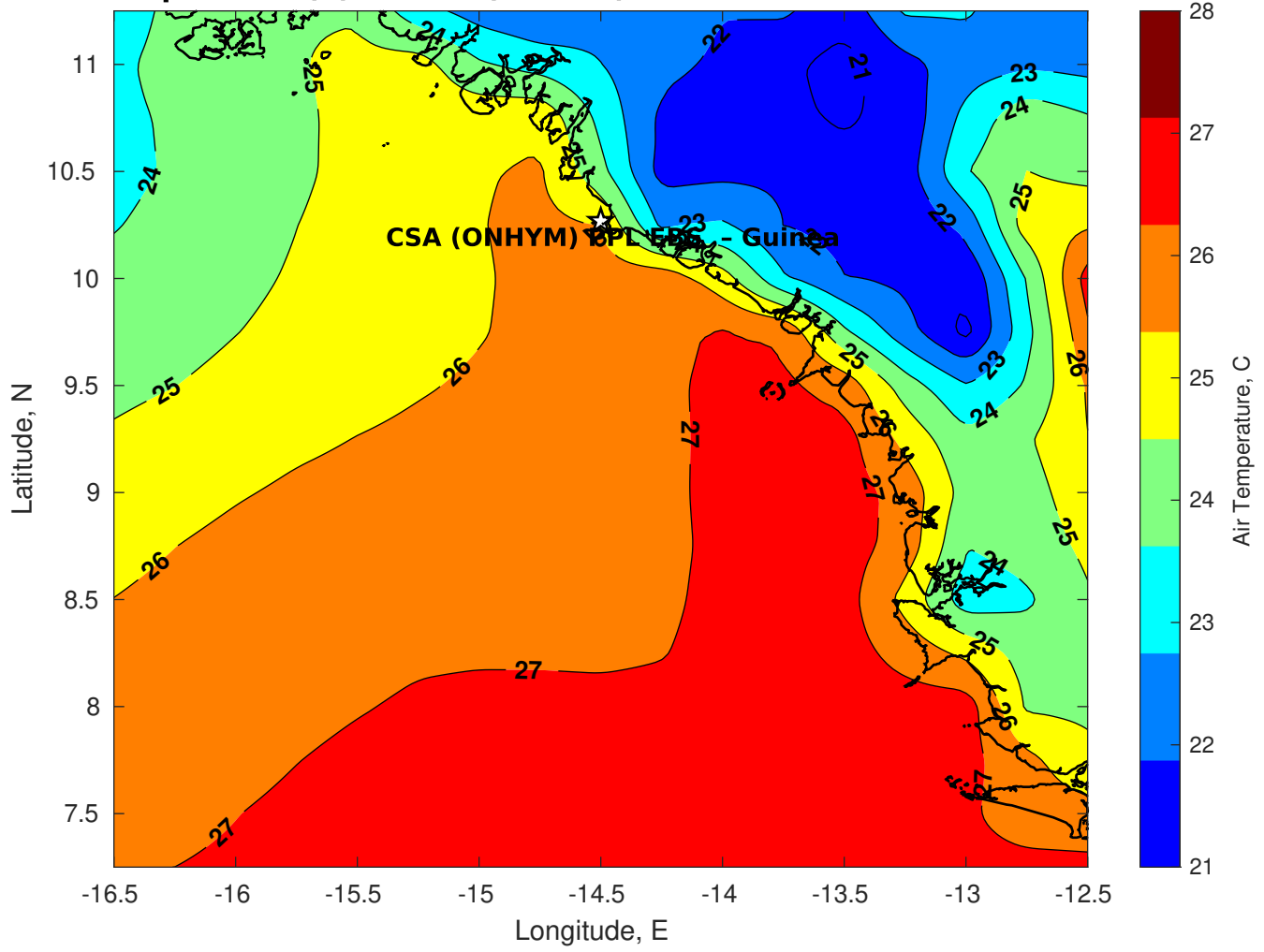
Air Temperature (C) for CSA (ONHYM) PPL EBS - Guinea at 20-Feb-2025
