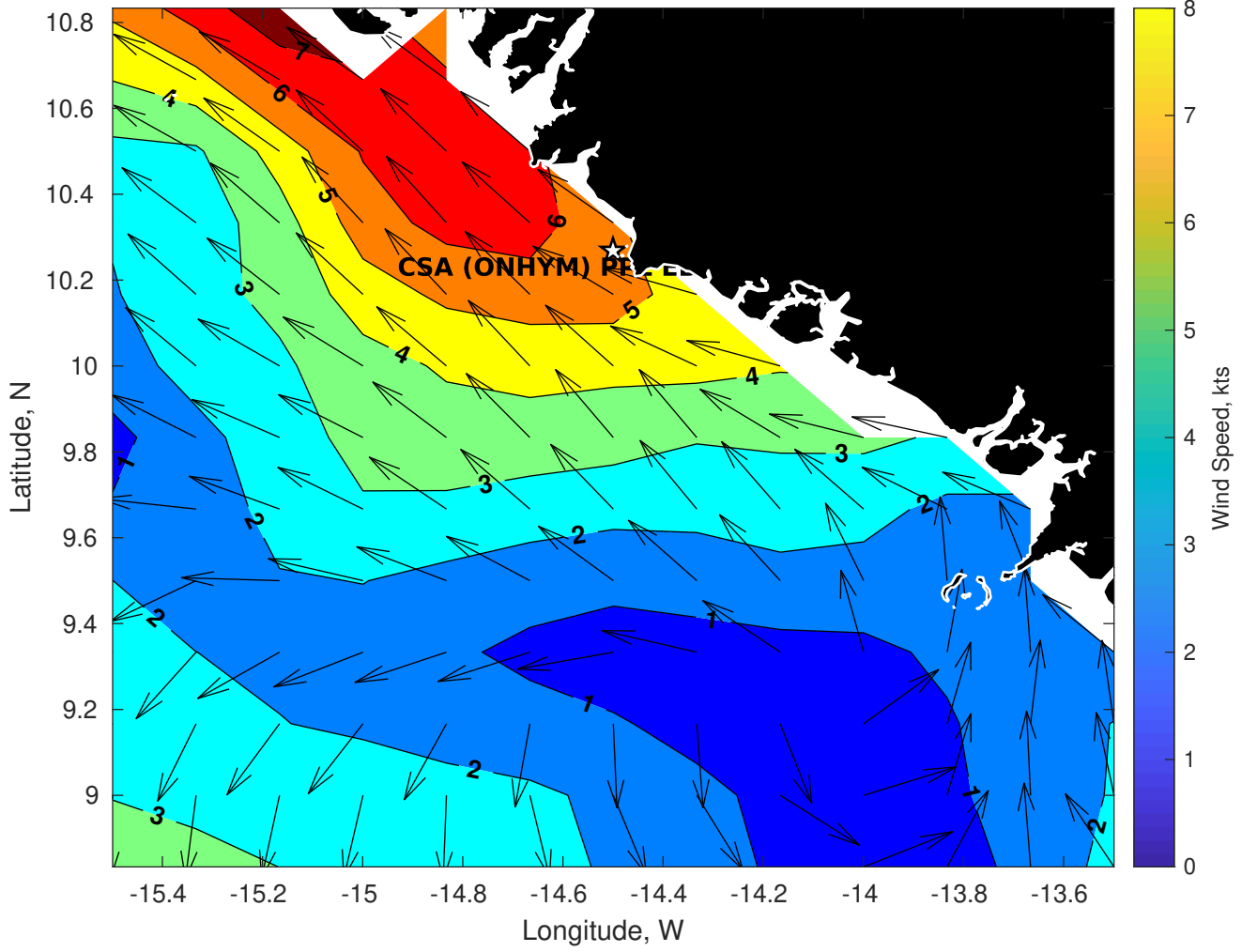
Winds (kts) for CSA (ONHYM) PPL EBS - Guinea at 20-Feb-2025 09:00:00
