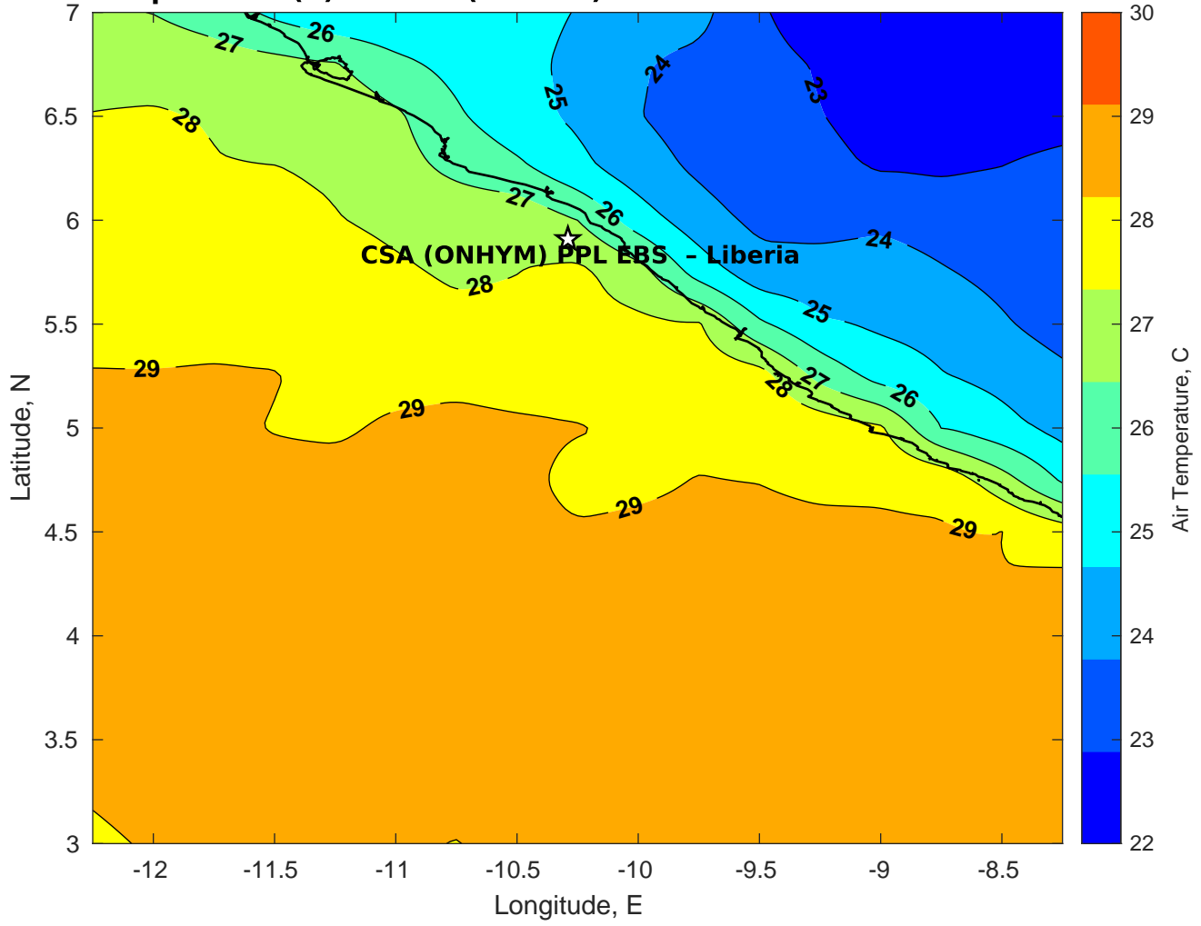
Air Temperature (C) for CSA (ONHYM) PPL EBS - Liberia at 20-Feb-2025
