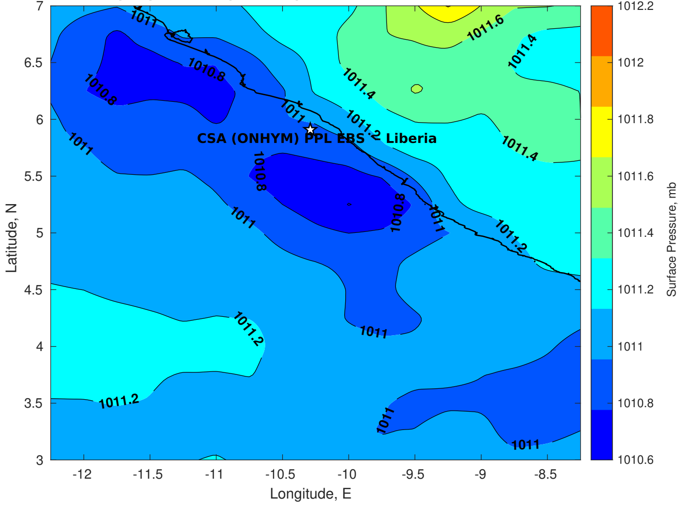
Surface Pressure (mb) for CSA (ONHYM) PPL EBS - Liberia at 21-Feb-2025 06:00:00
