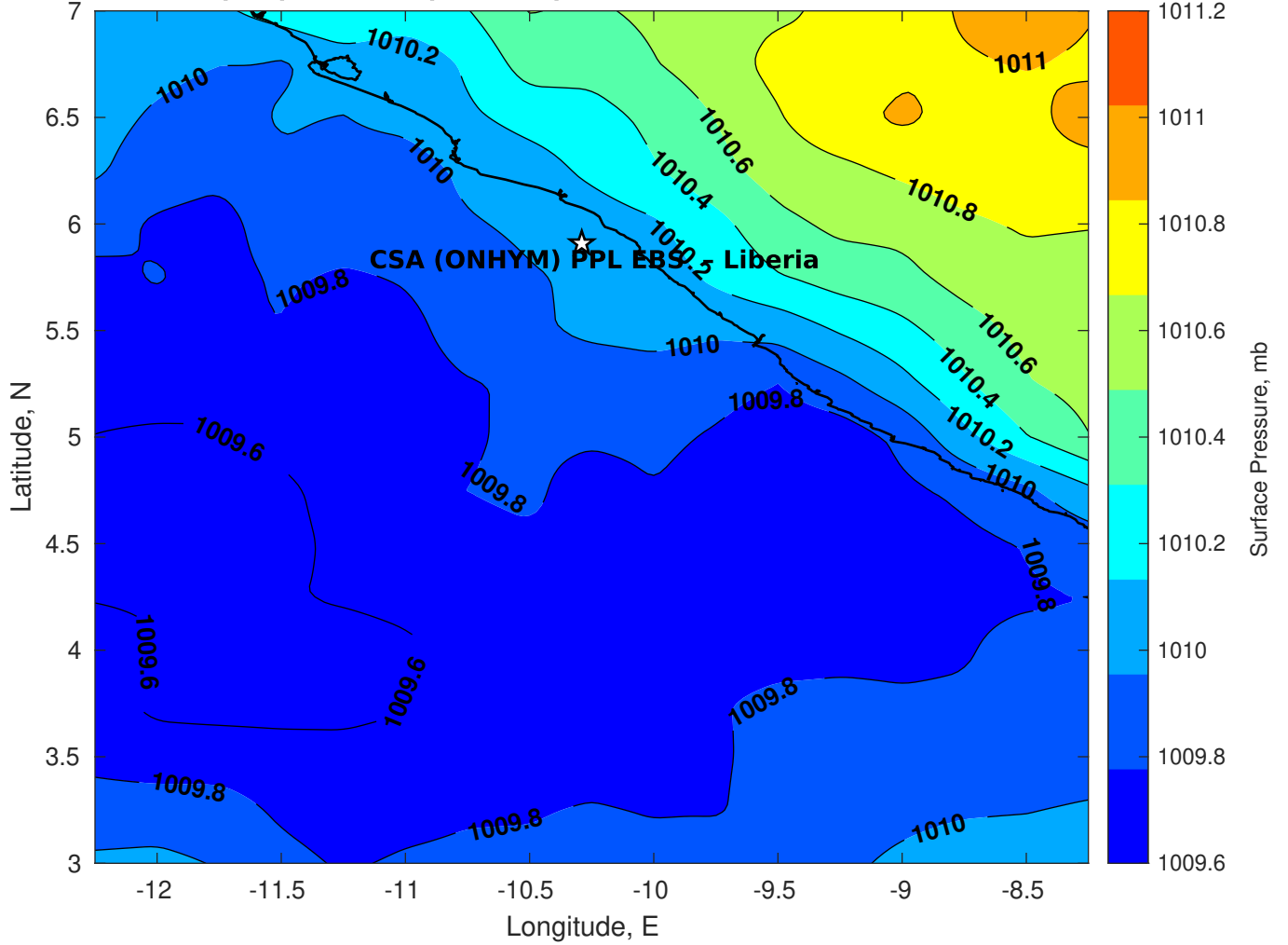
Surface Pressure (mb) for CSA (ONHYM) PPL EBS - Liberia at 22-Feb-2025 06:00:00
