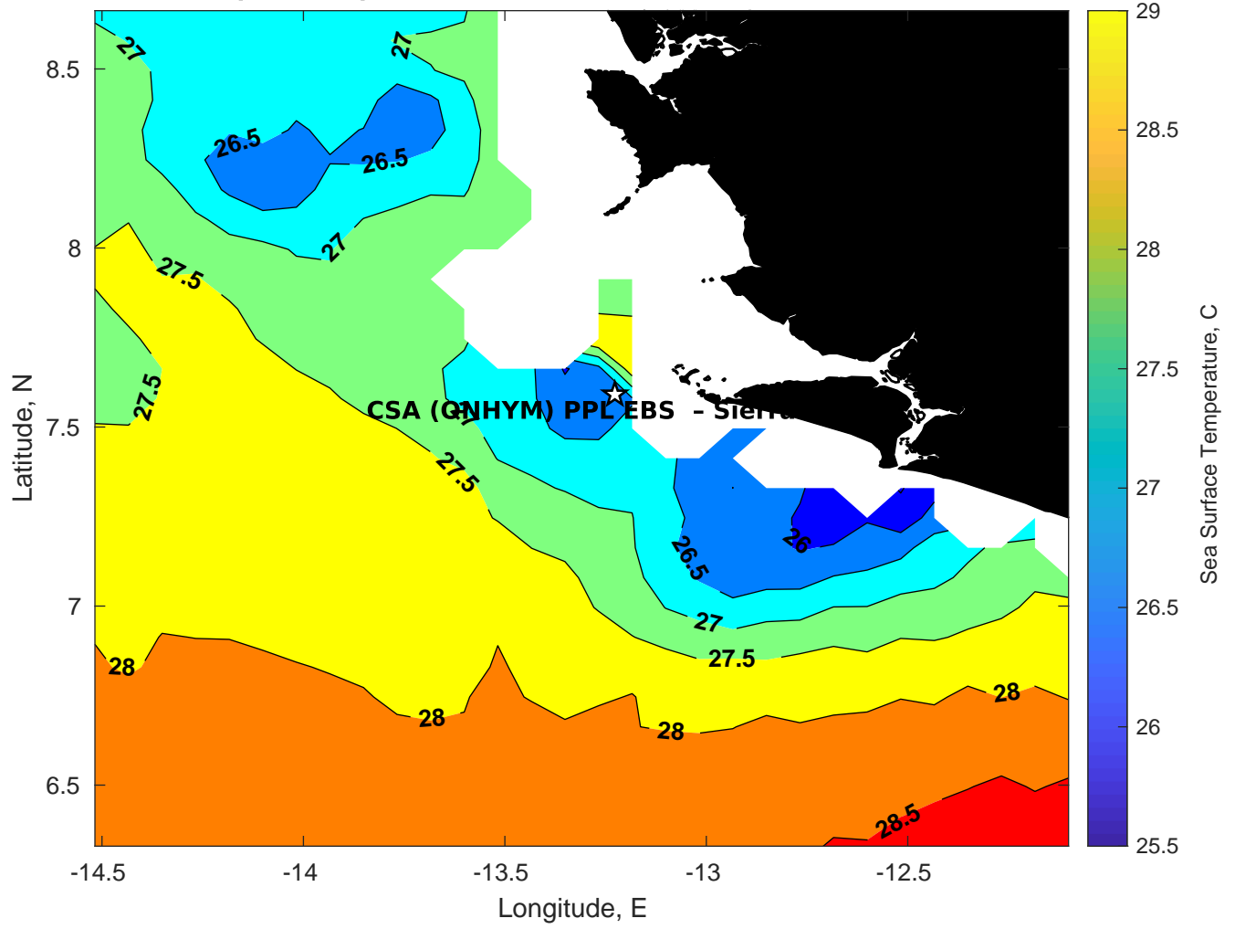
SST for CSA (ONHYM) PPL EBS - Sierra Leone at 19-Feb-2025 00:00:00
