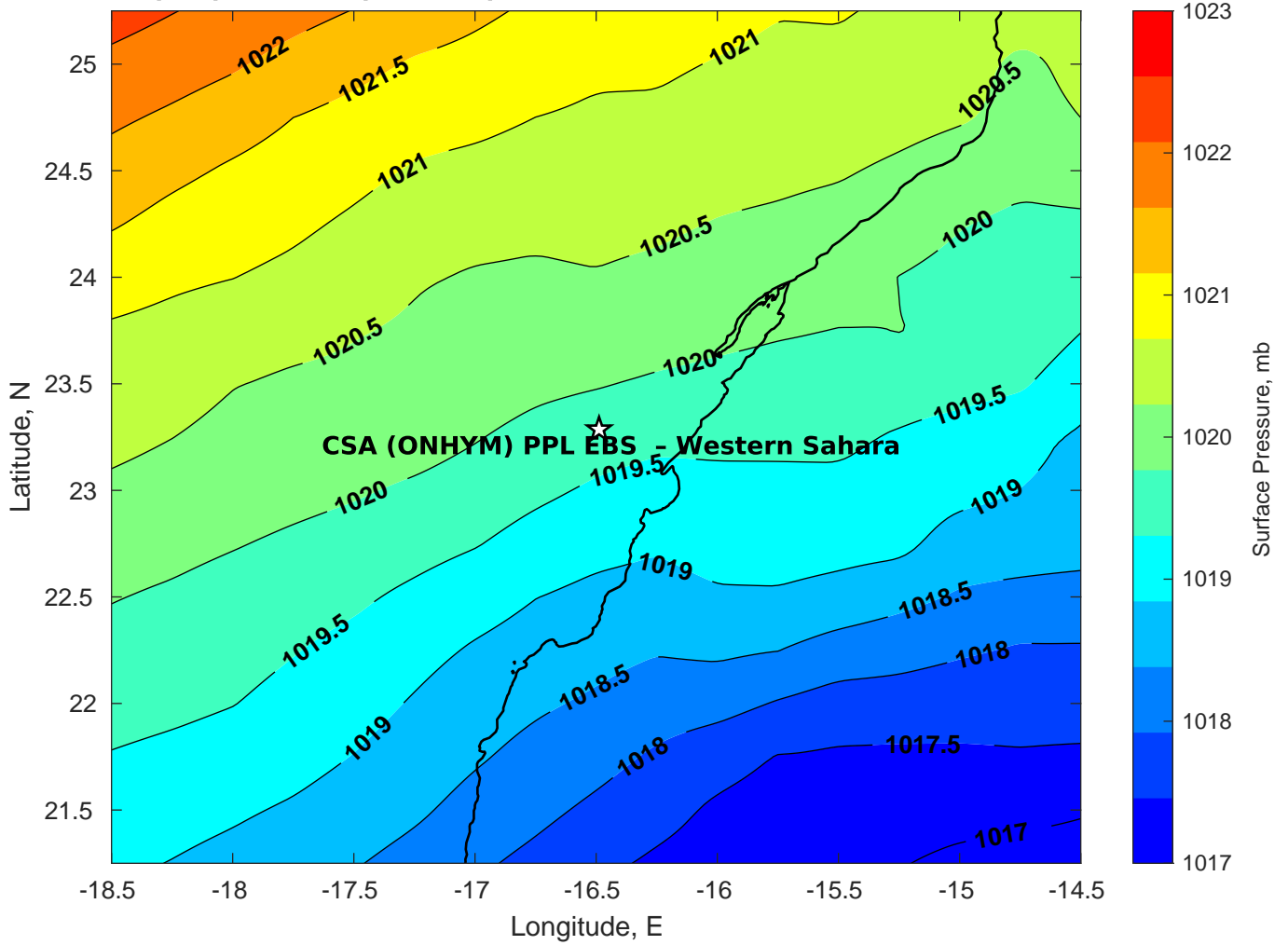
Surface Pressure (mb) for CSA (ONHYM) PPL EBS - Western Sahara at 21-Feb-2025 00:00:00
