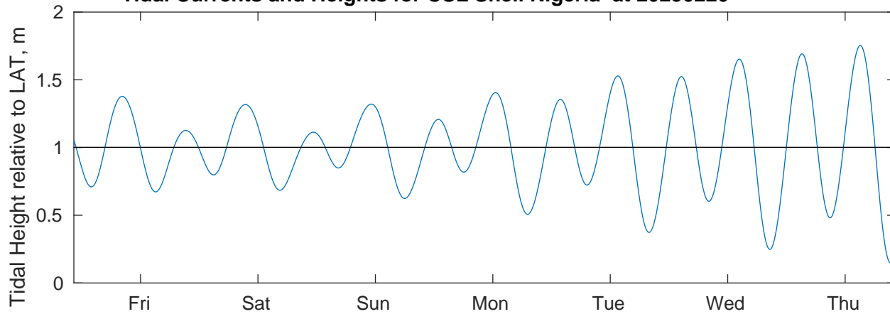
Tidal Currents and Heights for CSL Shell Nigeria at 20250220
