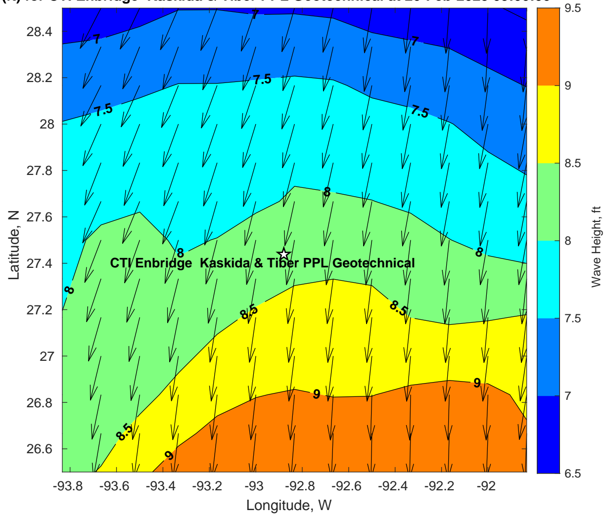
Wave Height (ft) for CTI Enbridge Kaskida & Tiber PPL Geotechnical at 20-Feb-2025 09:00:00
