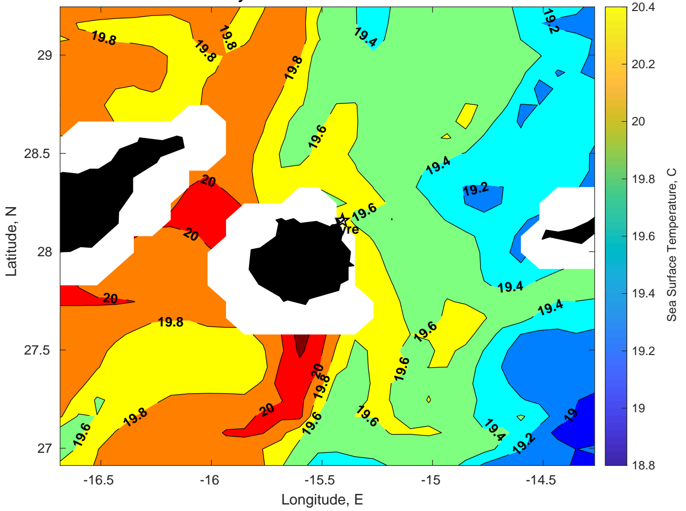
SST for Gyre at 19-Feb-2025 00:00:00
