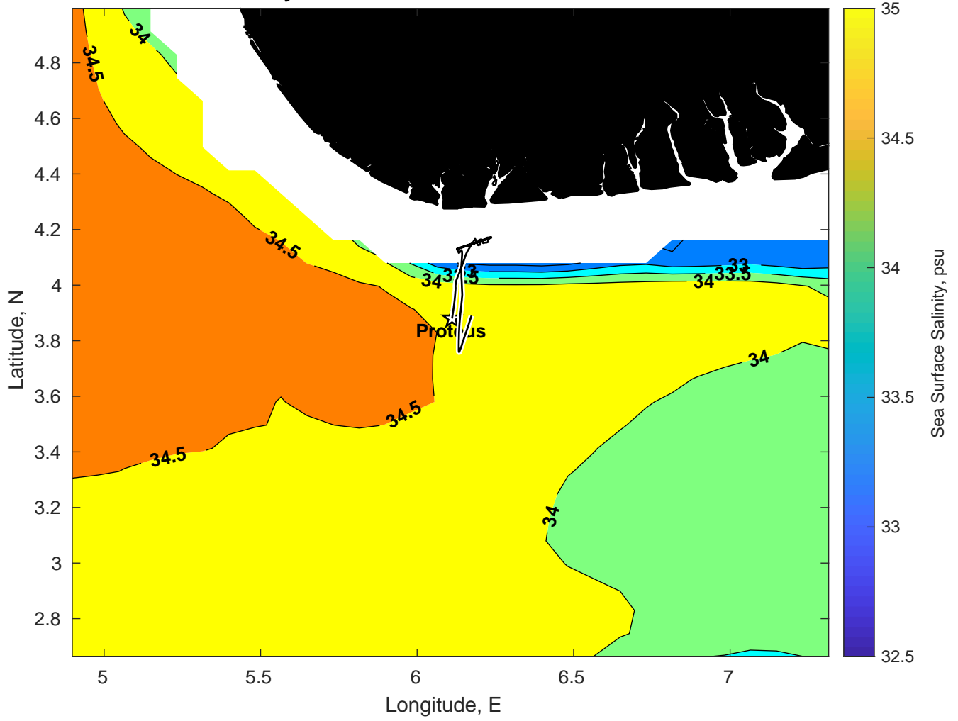
Surface Salinity for Proteus at 19-Feb-2025 00:00:00
