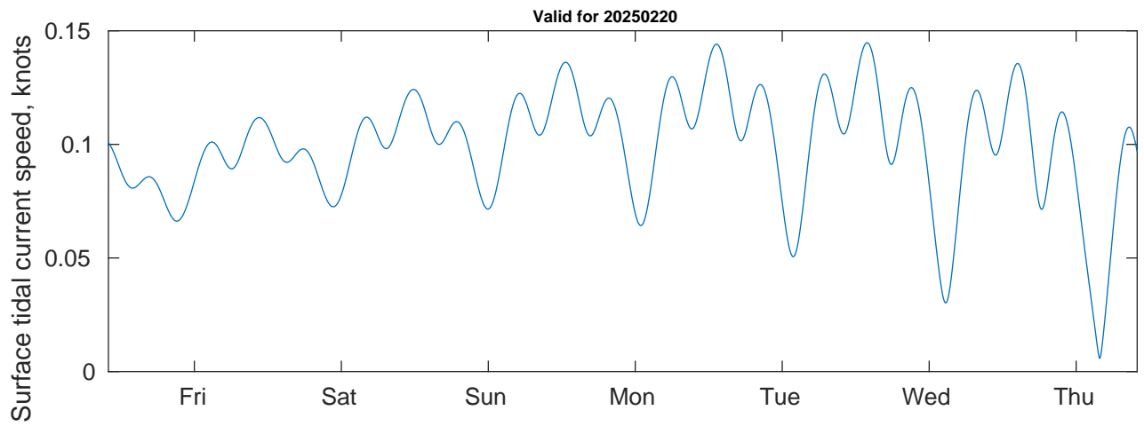
Tidal Currents and Heights for Shell Noches GC19 PPL Geotechnical at 20250220
