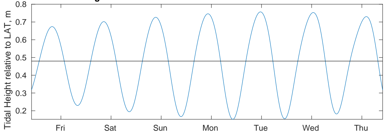
Tidal Currents and Heights for Shell Noches GC19 PPL Geotechnical at 20250220
