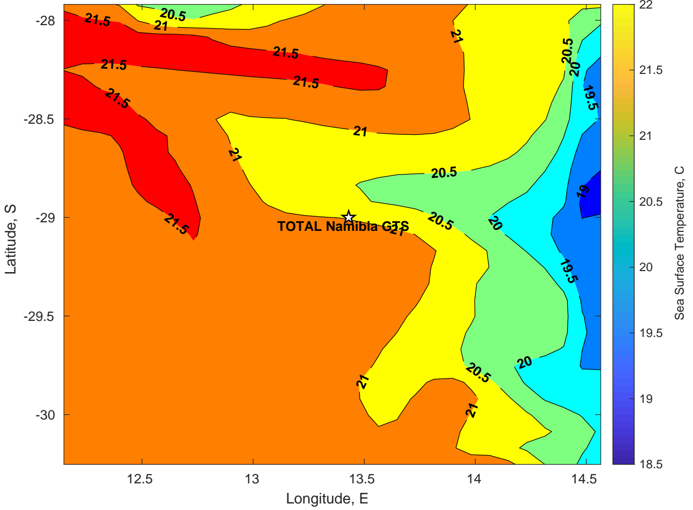
SST for TOTAL Namibia GTS at 19-Feb-2025 00:00:00
