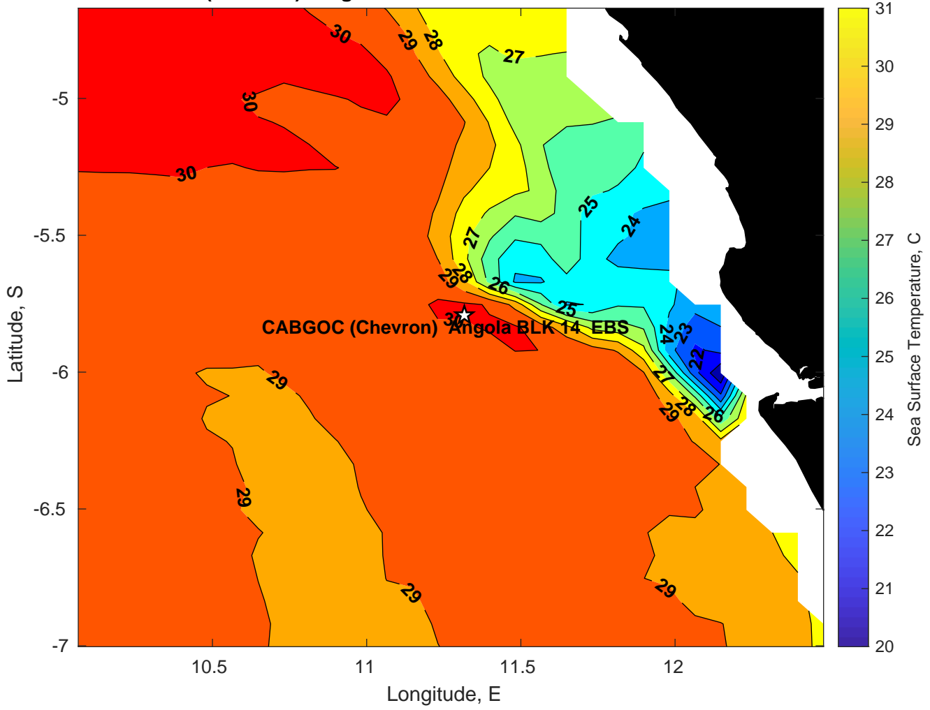
SST for CABGOC (Chevron) Angola BLK 14 EBS at 19-Feb-2025 00:00:00
