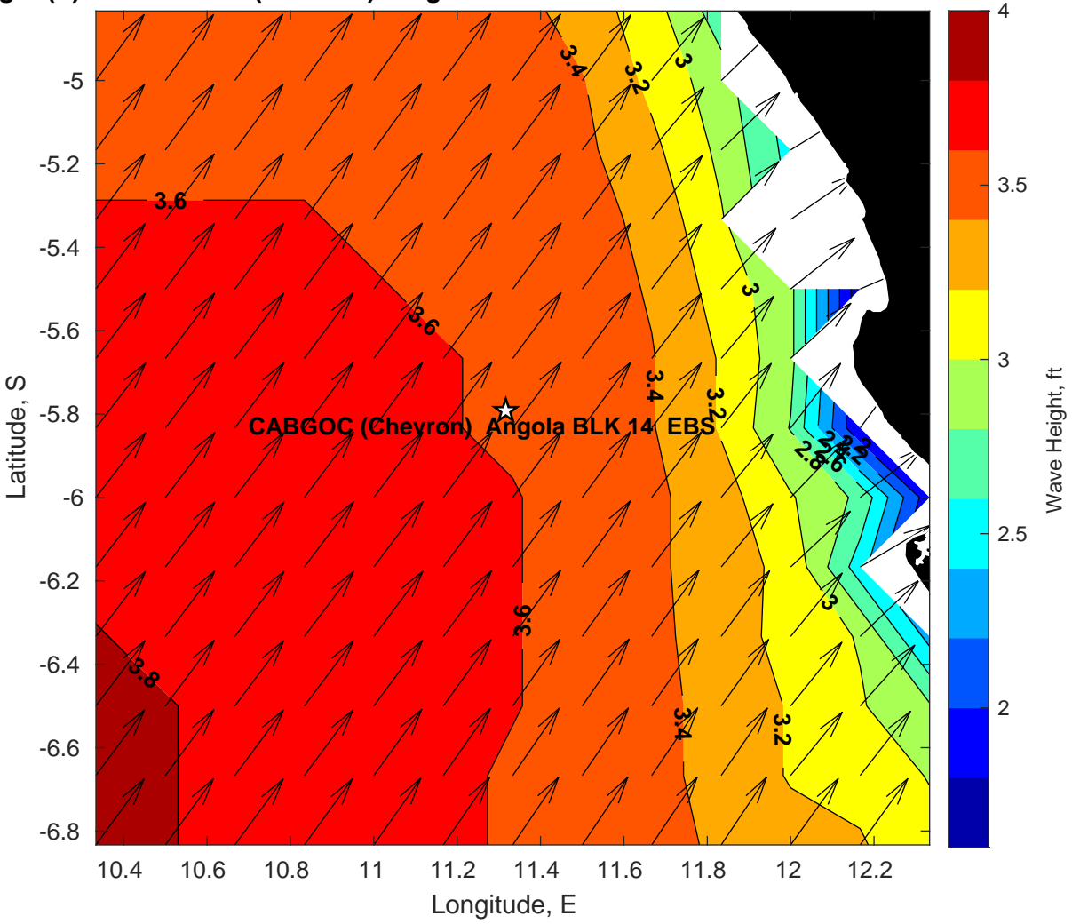
Wave Height (ft) for CABGOC (Chevron) Angola BLK 14 EBS at 21-Feb-2025 09:00:00
