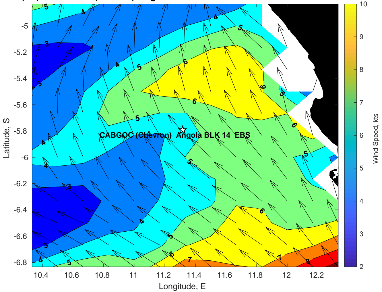
Winds (kts) for CABGOC (Chevron) Angola BLK 14 EBS at 21-Feb-2025 09:00:00
