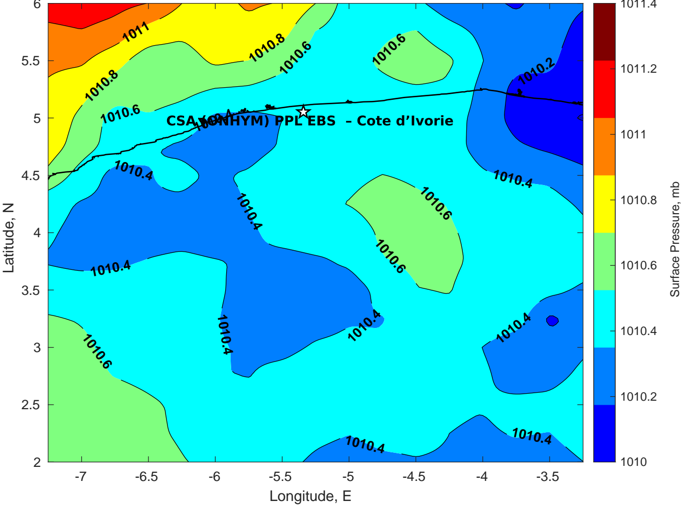
Surface Pressure (mb) for CSA (ONHYM) PPL EBS - Cote d'Ivoire at 21-Feb-2025 06:00:00
