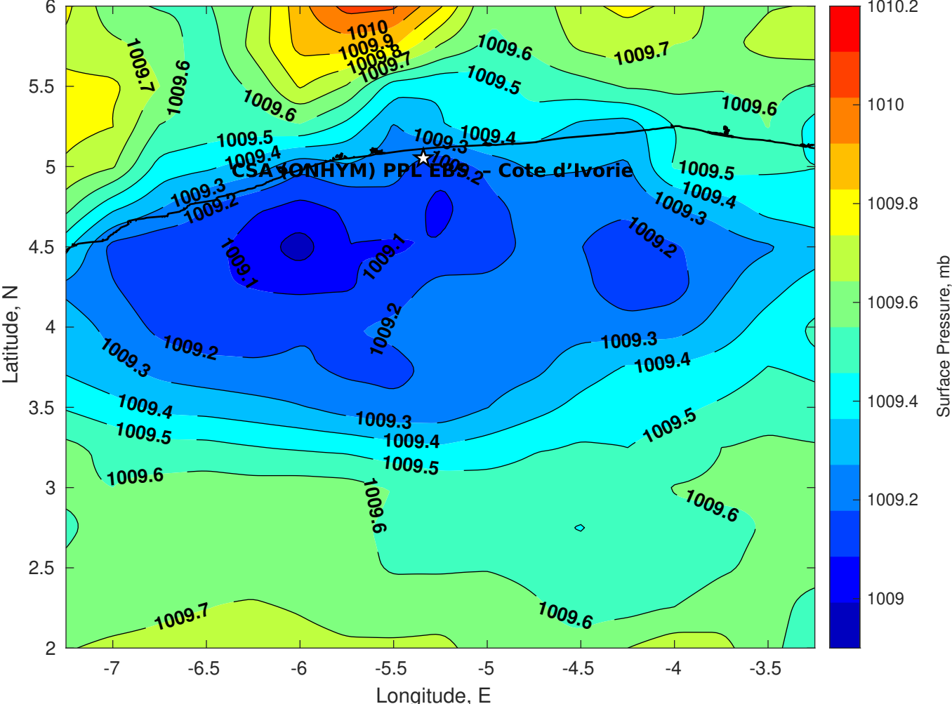
Surface Pressure (mb) for CSA (ONHYM) PPL EBS - Cote d'Ivoire at 22-Feb-2025 06:00:00
