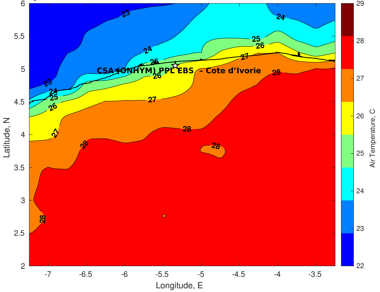
Air Temperature (C) for CSA (ONHYM) PPL EBS - Cote d'Ivoire at 21-Feb-2025
