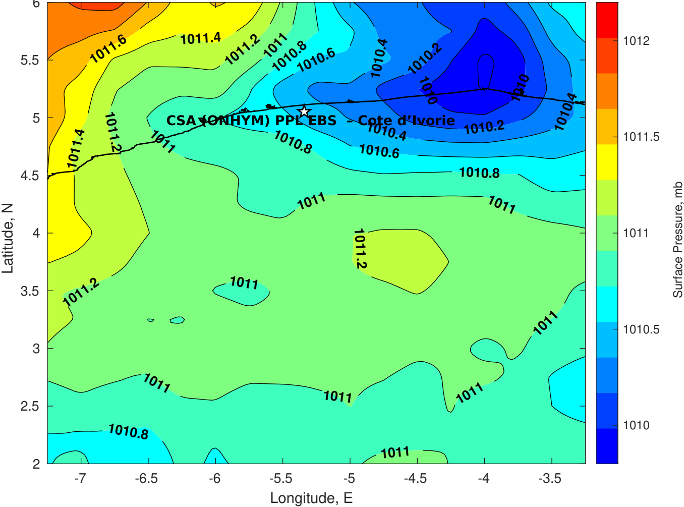
Surface Pressure (mb) for CSA (ONHYM) PPL EBS - Cote d'Ivoire at 23-Feb-2025 06:00:00
