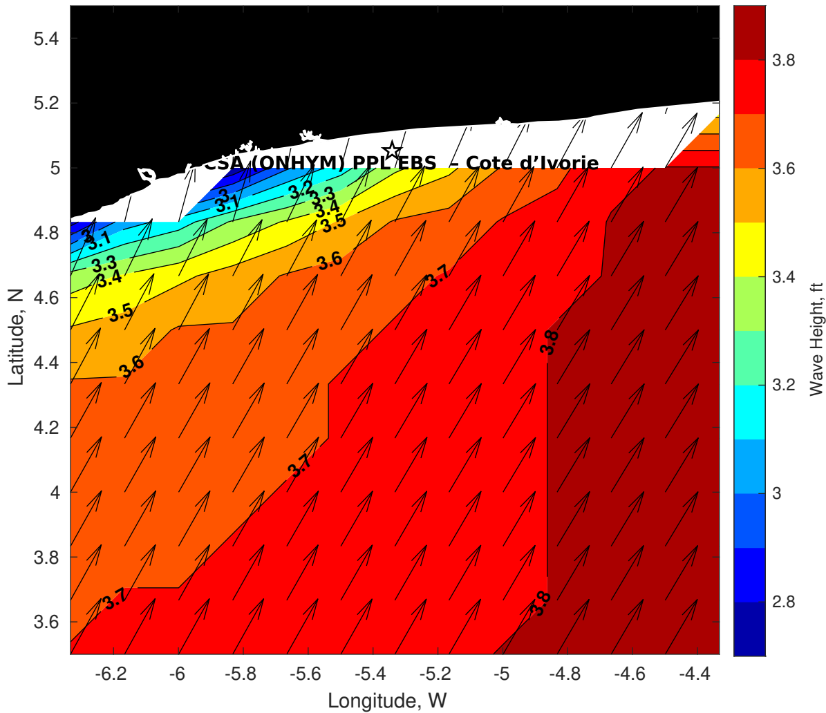
Wave Height (ft) for CSA (ONHYM) PPL EBS - Cote d'Ivoire at 21-Feb-2025 09:00:00
