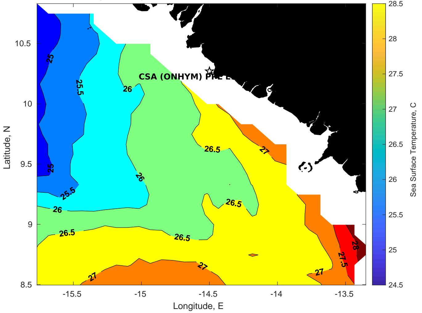
SST for CSA (ONHYM) PPL EBS - Guinea at 19-Feb-2025 00:00:00
