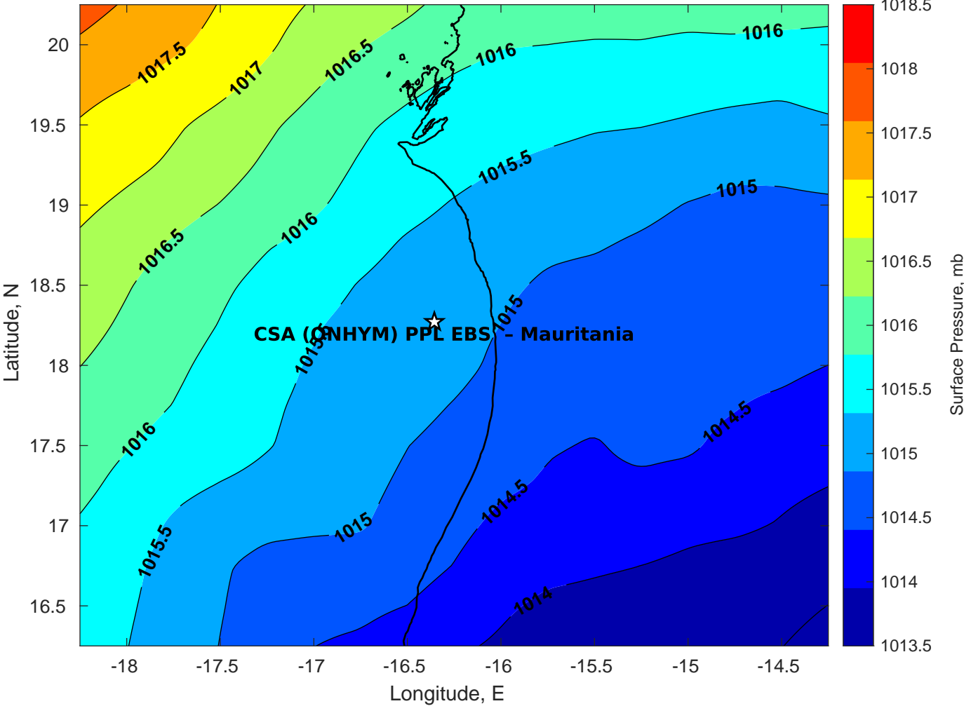
Surface Pressure (mb) for CSA (ONHYM) PPL EBS - Mauritania at 21-Feb-2025 00:00:00
