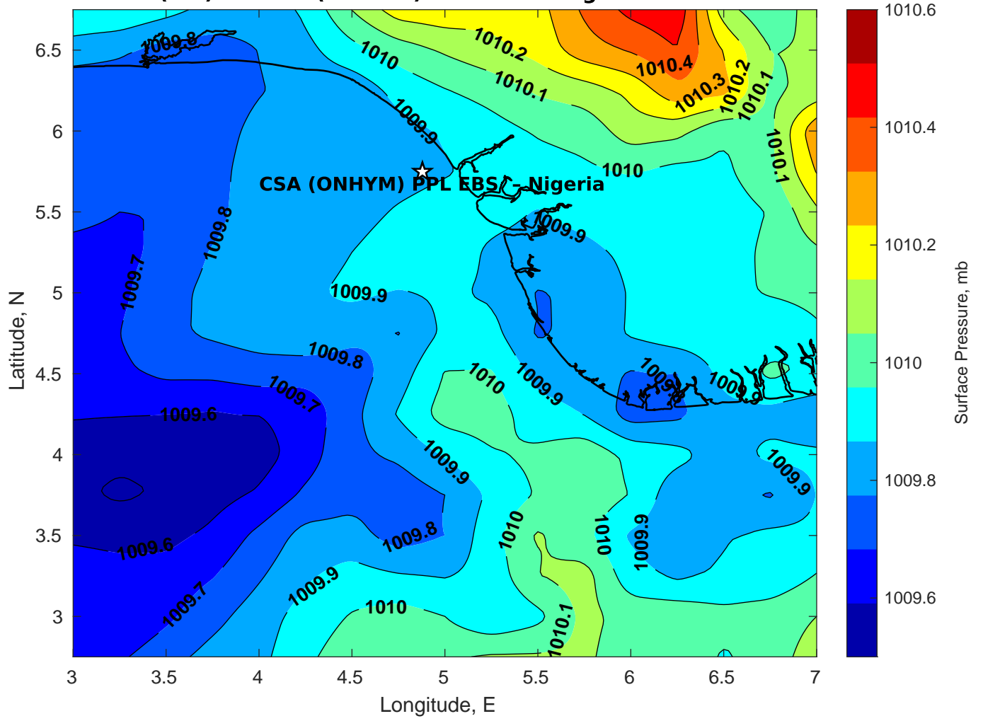
Surface Pressure (mb) for CSA (ONHYM) PPL EBS - Nigeria at 21-Feb-2025 06:00:00
