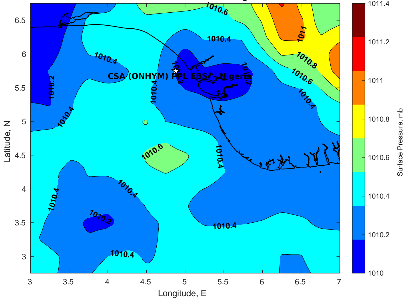
Surface Pressure (mb) for CSA (ONHYM) PPL EBS - Nigeria at 23-Feb-2025 06:00:00
