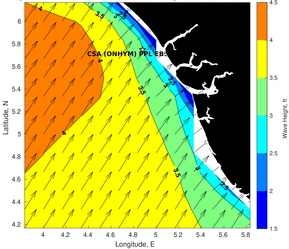
Wave Height (ft) for CSA (ONHYM) PPL EBS - Nigeria at 21-Feb-2025 09:00:00
