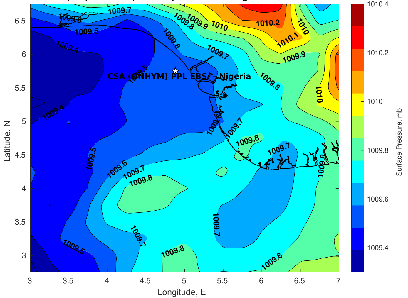
Surface Pressure (mb) for CSA (ONHYM) PPL EBS - Nigeria at 22-Feb-2025 06:00:00
