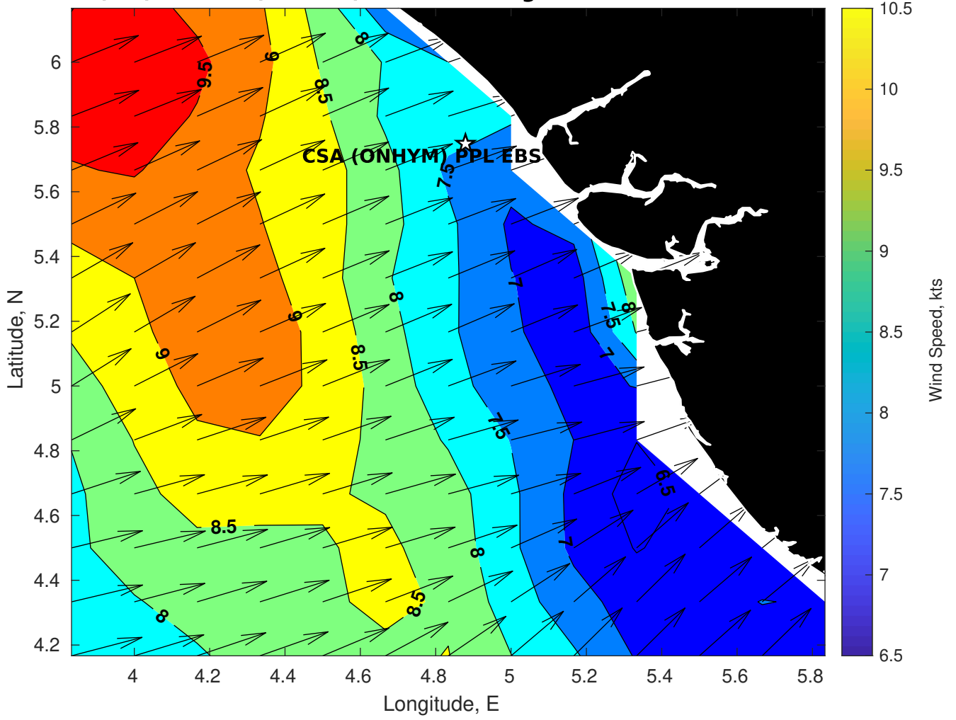
Winds (kts) for CSA (ONHYM) PPL EBS - Nigeria at 21-Feb-2025 09:00:00
