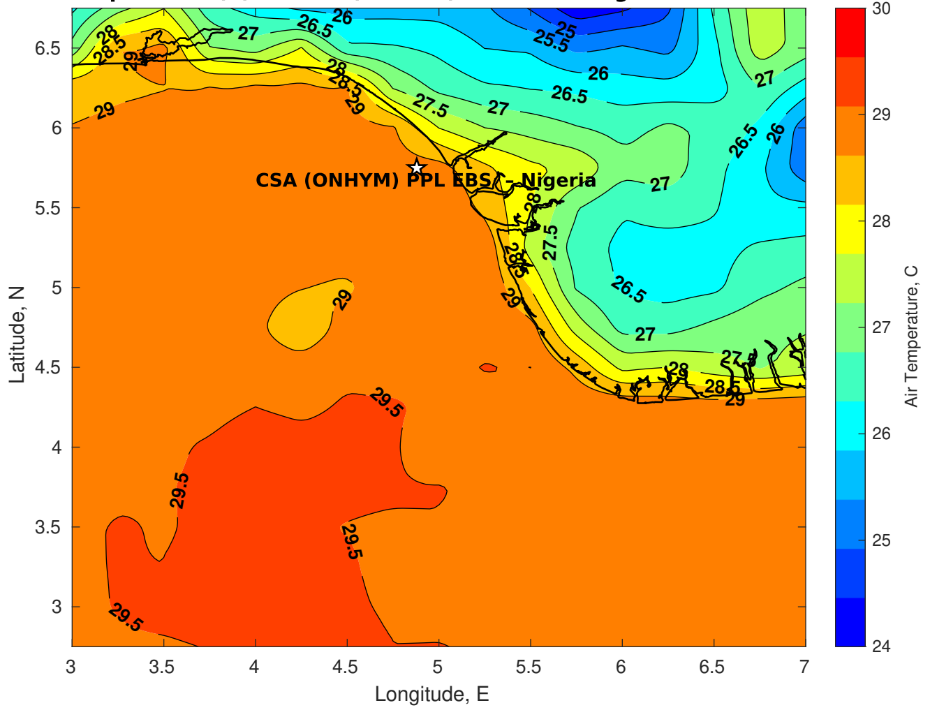
Air Temperature (C) for CSA (ONHYM) PPL EBS - Nigeria at 21-Feb-2025
