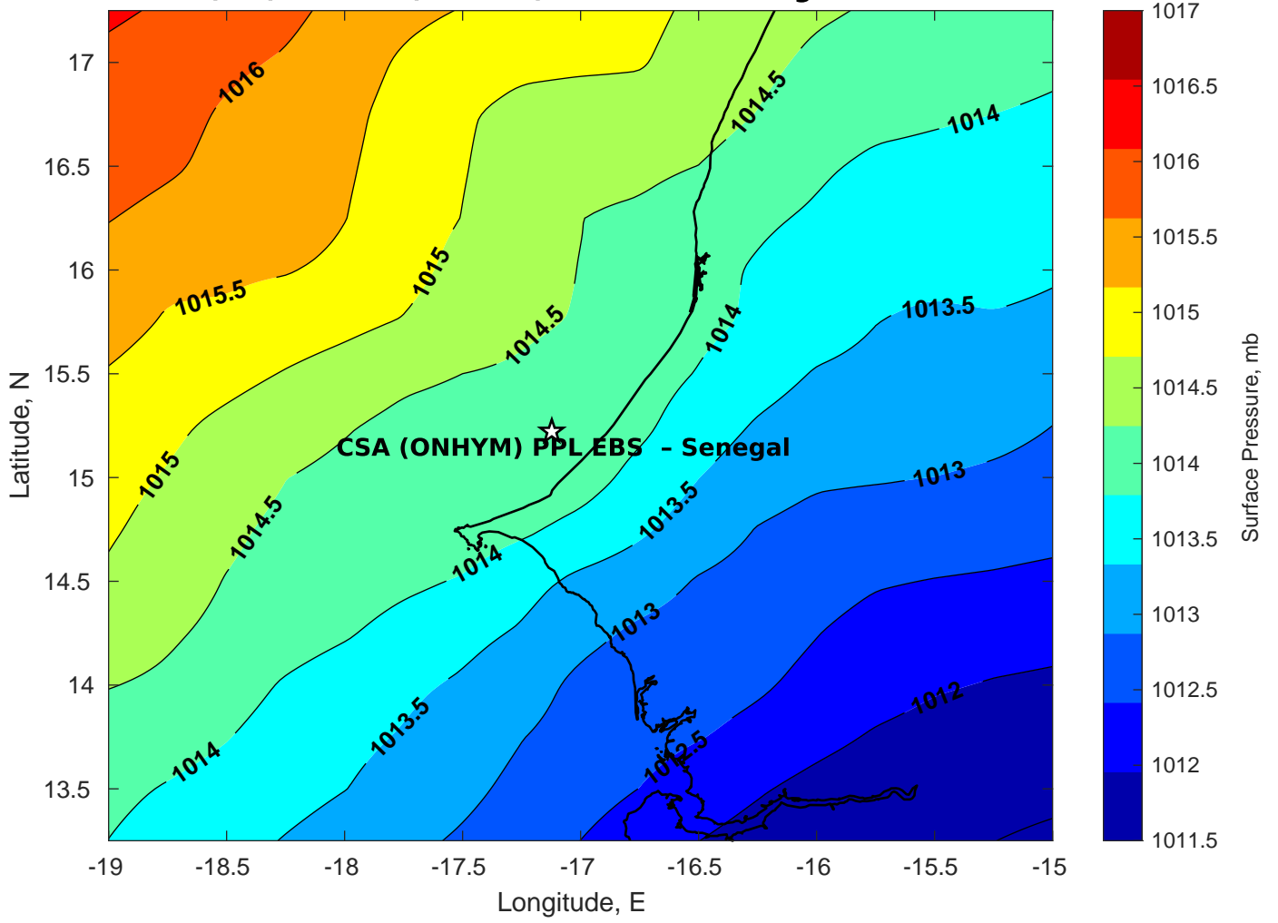
Surface Pressure (mb) for CSA (ONHYM) PPL EBS - Senegal at 21-Feb-2025 00:00:00
