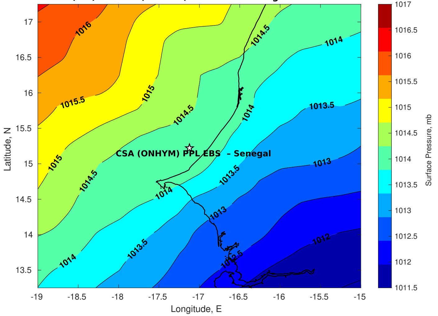
Surface Pressure (mb) for CSA (ONHYM) PPL EBS - Senegal at 21-Feb-2025 00:00:00
