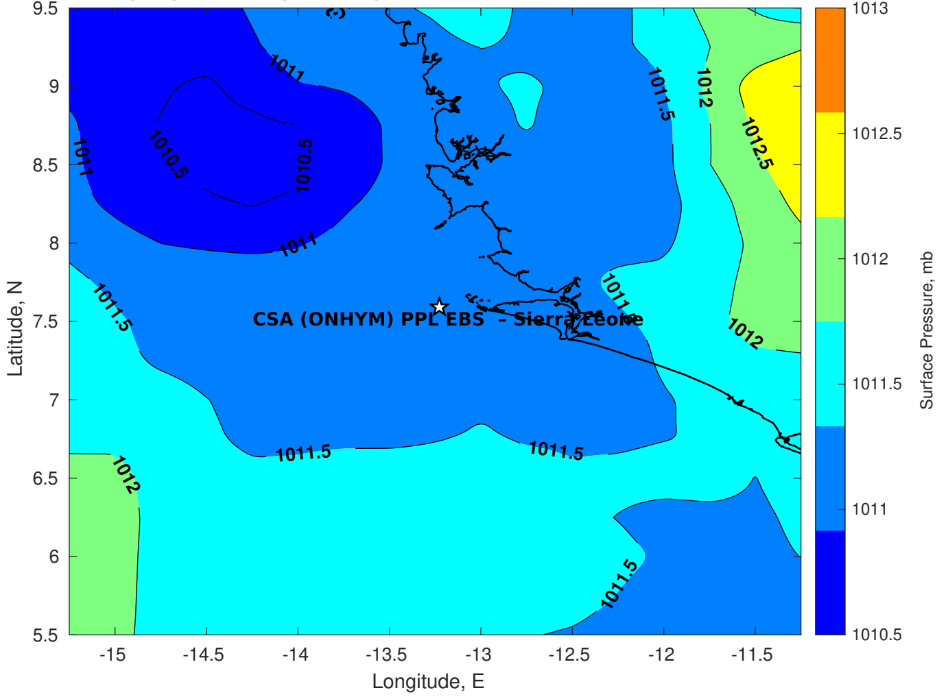
Surface Pressure (mb) for CSA (ONHYM) PPL EBS - Sierra Leone at 23-Feb-2025 00:00:00
