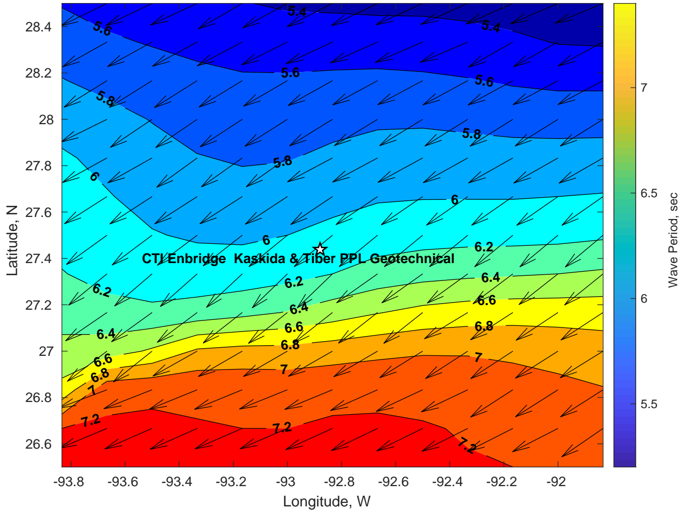
Wave Period (sec) for CTI Enbridge Kaskida & Tiber PPL Geotechnical at 21-Feb-2025 09:00:00
