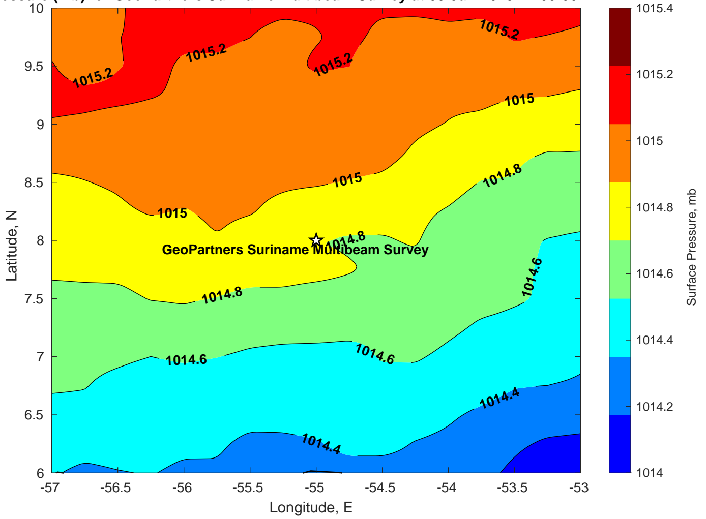
Surface Pressure (mb) for GeoPartners Suriname Multibeam Survey at 08-Jan-2025 12:00:00
