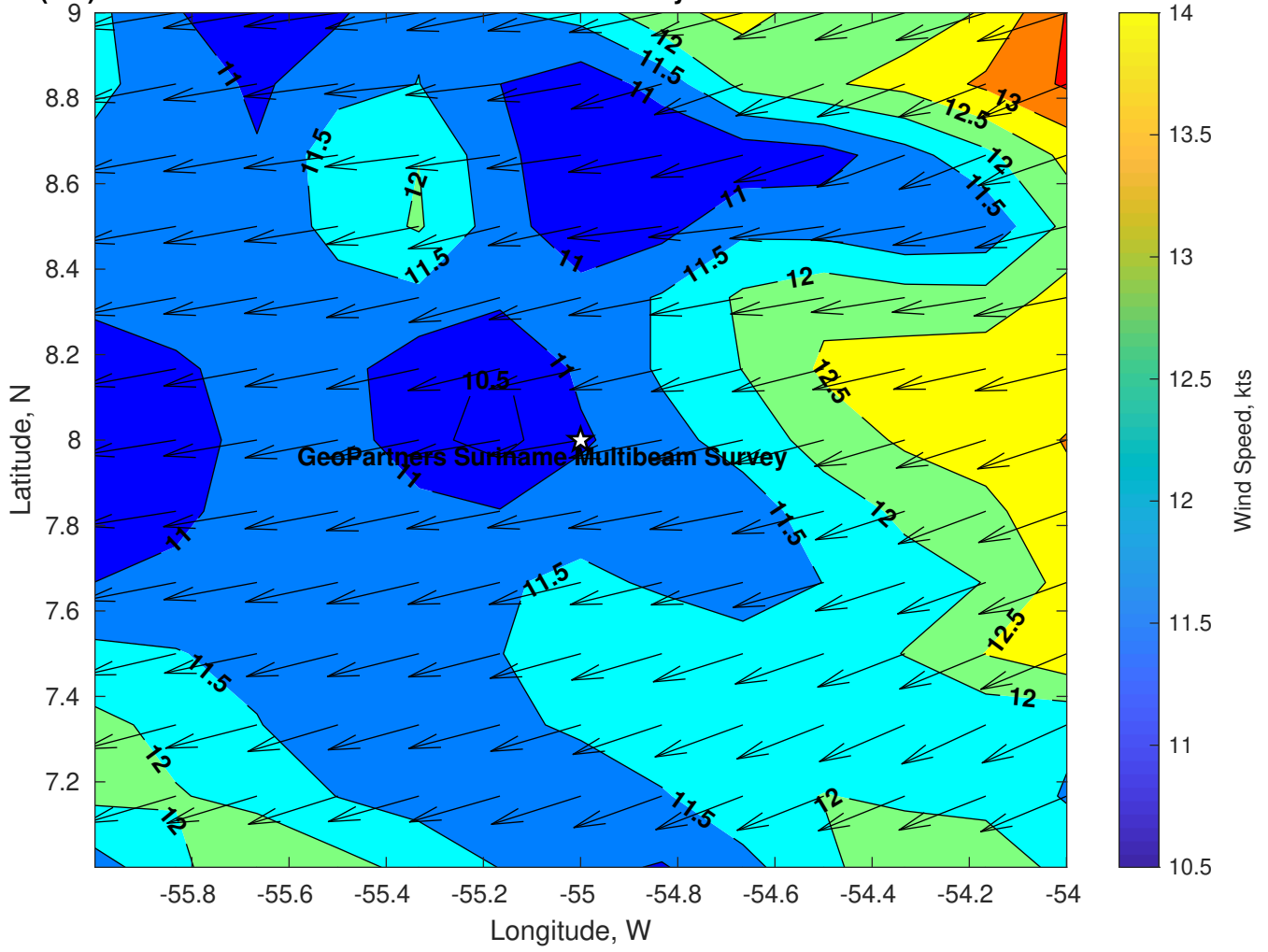
Winds (kts) for GeoPartners Suriname Multibeam Survey at 08-Jan-2025 21:00:00
