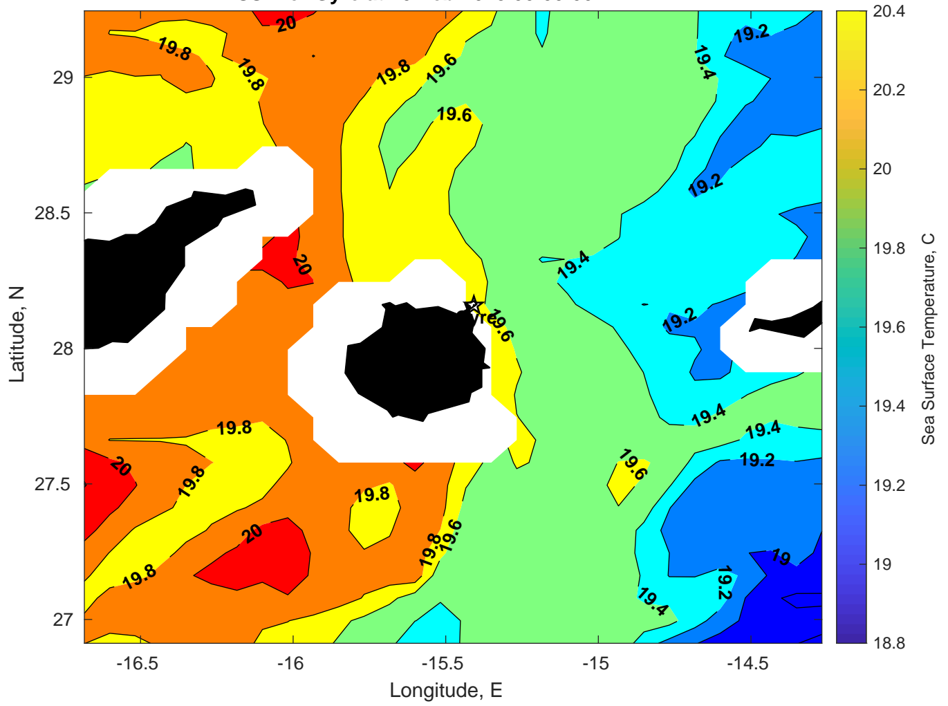
SST for Gyre at 20-Feb-2025 00:00:00
